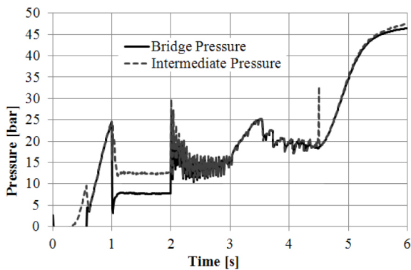
Figure 23. Valve - Intermediate and Bridge Pressure
