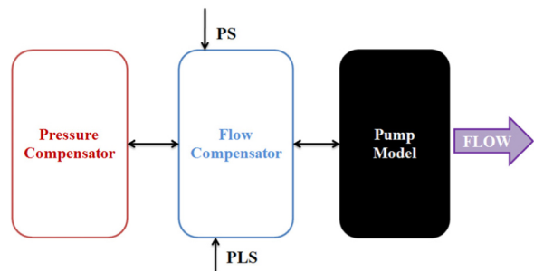
Figure 2. Gray Box modeling methodology
