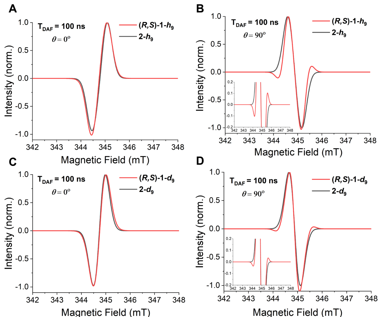
Fig. 4. Simulations of the TREPR spectra with a minimal model of the SCRP. The model places one hydrogen nuclear spin- \frac{1}{2} on both PXX ^{+} and NDI ^{-} (A, B) or only on NDI ^{-} (C, D). The nuclear spins are coupled to each radical with isotropic hyperfine couplings a_{\text{NDI}} = 6.3 MHz and a_{\text{PXX}} = 10 MHz. Insets: the simulations are shown with their intensities expanded to highlight features characteristic of CISS. The complete list of simulation parameters is given in table S7.
