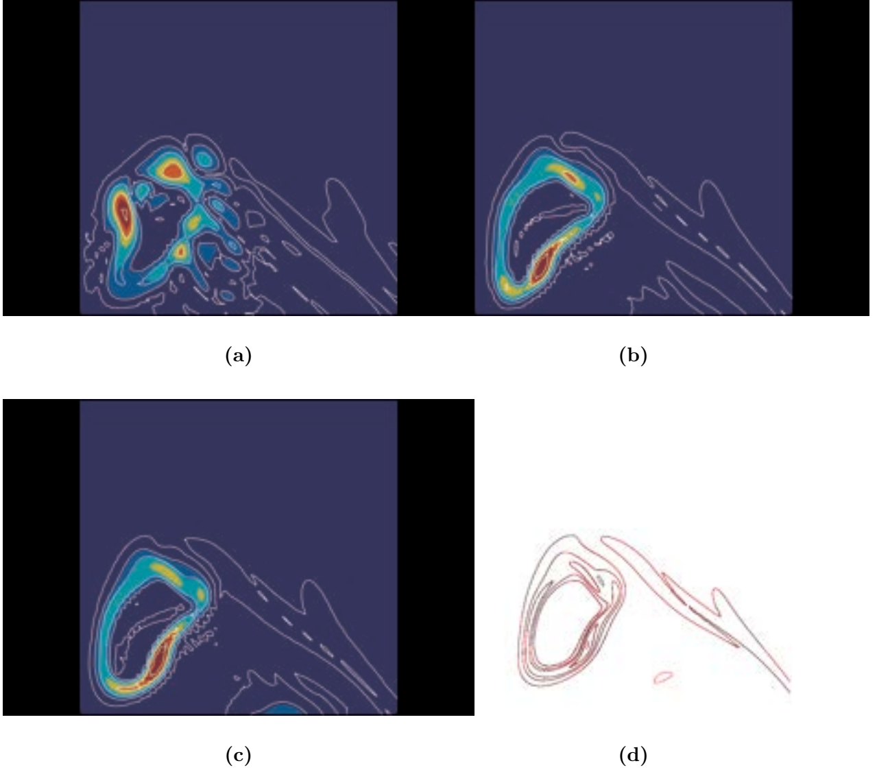
Figure 4.19 Vorticity contours for \omega = 1, 5, 10, 20, 30 at x = -0.5 for the (a) 2nd, (b) 4th and (c) 6th order schemes for the Taylor-Green Vortex at Re=1,600 . (d) Reference solution in [253] .
