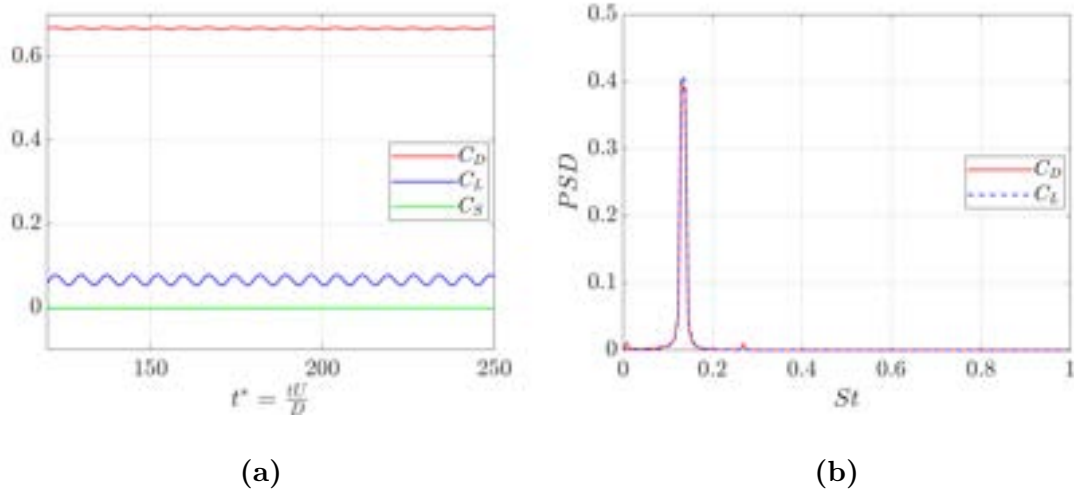
Figure 6.2 (a) Time histories and (b) normalized power spectral densities of the aerodynamic coefficients for the flow past a sphere at Re = 300 .
