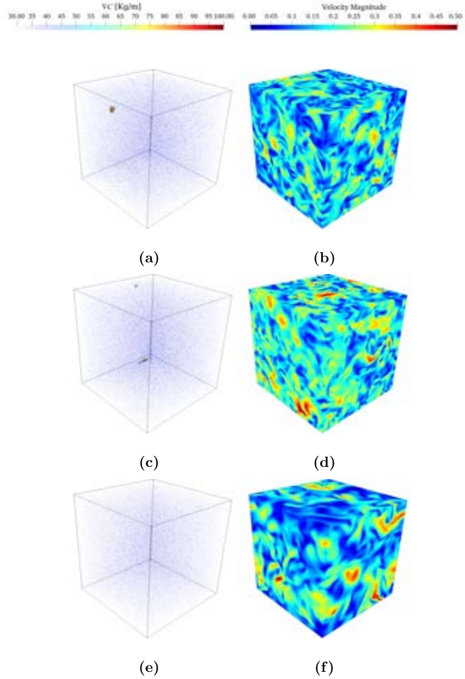
Figure 4.16 Contours of \nabla C (left) and velocity (right) at t = 11 for the forced isotropic turbulent cases with A = 0.3 . (a), (b) Lagrangian SPH; (c), (d) Lagrangian SPH with PST and ALE terms; (e), (f) Lagrangian SPH with PST and without ALE terms.
