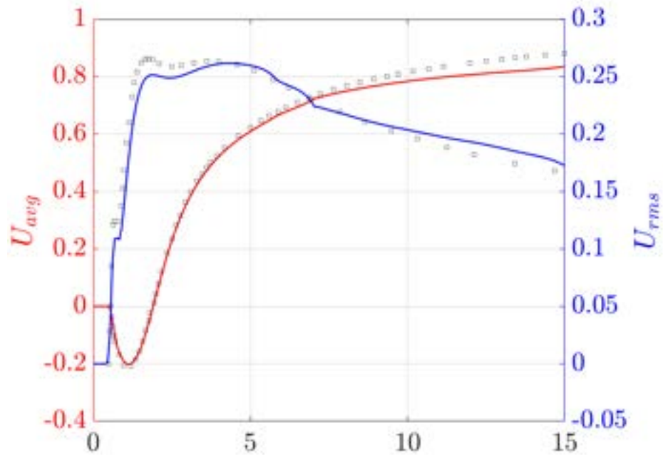
Figure 6.4 Comparison of the average and root-mean-square values of the streamwise velocity along the wake centerline with the numerical results in [242]
