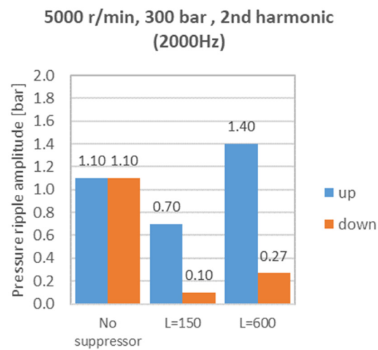
Figure 24. Pressure amplitude at different pipe lengths, Second harmonic, 5000 r/min.
