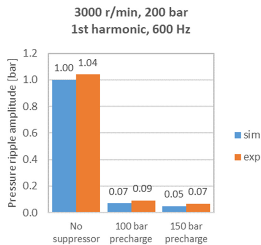
Figure 9. First harmonic, 200 bar, n = 3000 r/min.
