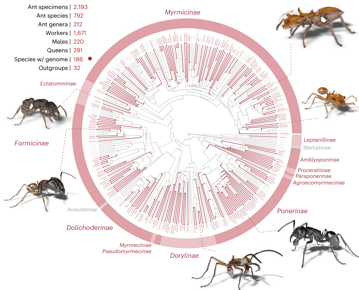
Fig. 2 | The diverse set of species and genera across the ant tree of life covered by Antscan. The ant phylogeny with genera sampled in Antscan displayed in red and missing genera in gray. A dot at the end of a genus branch indicates that at least one genome from a species within that genus is sequenced. Examples of 3D models derived from the micro-CT scans shown clockwise from the
