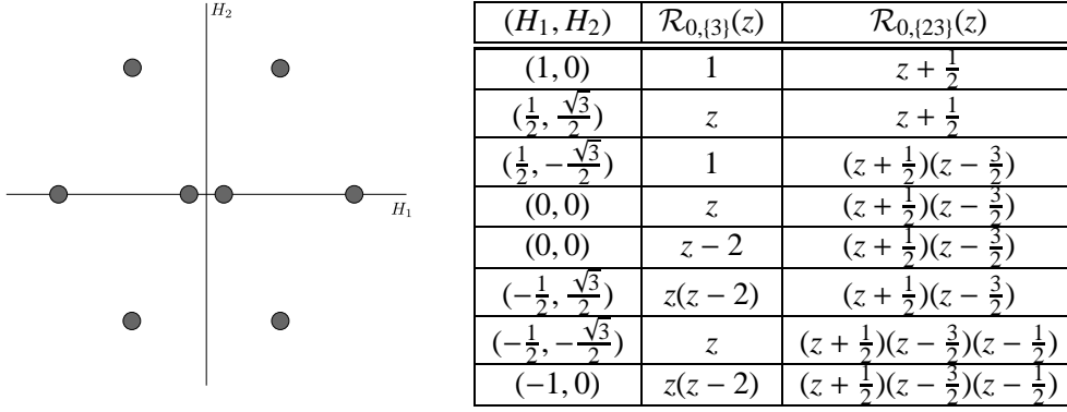
Figure 1: Polynomial structure of the \mathcal{R} -operators using the normalization in [7].
