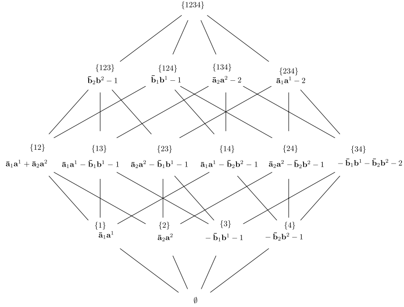
Figure 2: Hasse diagramm for \mathfrak{su}(2,2) including the shifted weights of the subalgebra \hat{\ell}_1^I - \gamma according to (C.18).
