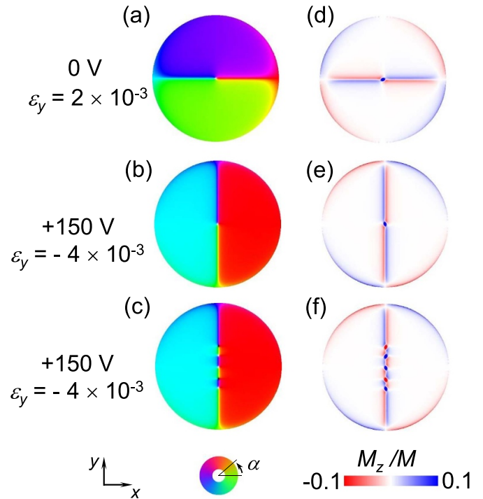
Figure 5. Micromagnetic modelling of a Ni disc under strain-mediated voltage control. Maps of (a)–(c) in-plane magnetization direction \alpha and (d)–(f) out-of-plane magnetization M_z describe the near-surface disc magnetization for the uniaxial strain \varepsilon_y that we identify with the application of (a), (d) 0 V and (b), (e) +150 V. Panels (c) and (f) assume the same strain as panels (b) and (e), and show a multivortex state whose energy is 0.2% higher. The magnitude of the local magnetization is denoted M .
