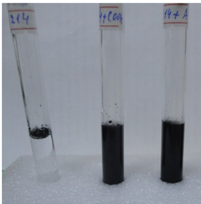
Figure S1: Dispersibility behavior in water of (from left to right): pristine MWCNTs, COOH-MWCNT and NH 2 -C 2 -MWCNT. The picture was taken four weeks after dispersion of the material in water by sonication.
