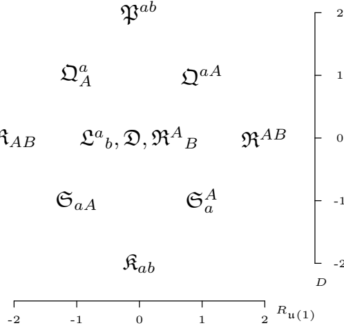
Figure 1: The generators of \mathfrak{osp}(6|4) can be arranged according to their dilatation charge and their \mathfrak{u}(1) charge under \mathfrak{K}_C^C .
