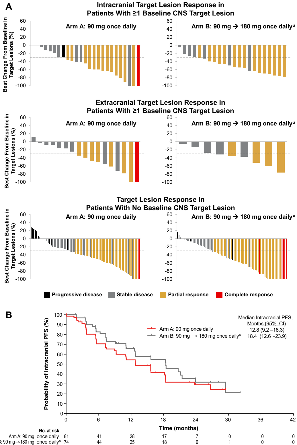
Figure 3. Brigatinib intracranial efficacy and best target lesion response in crizotinib-refractory ALK-positive NSCLC. (A) The best percentage change from baseline in the sum of the longest diameters of intracranial and extracranial target lesions is reported in patients who had at least one target brain lesion at baseline, as assessed by investigators. The dotted line at -30\% indicates the threshold for partial response per RECIST version 1.1. (B) Intracranial PFS is shown for patients with any brain metastases at baseline, as assessed by an IRC ( n = 81 , arm A; n = 74 , arm B). Of the 81 evaluable patients in arm A, 40 (49%) had an event; of the 74 evaluable patients in arm B, 30 (41%) had an event. (C) Investigator-assessed PFS by best target lesion shrinkage and (D) IRC-assessed PFS by best target lesion shrinkage in patients with one or more evaluable response
