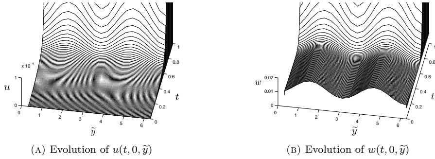
FIGURE 4. Evolution of (u, w) solution of the linear problem (3.23) (with \mathbf{f} = \mathbf{0} and \mathbf{h} = \mathbf{0} ) for \theta_i = 0.75 , Le = 0.3 < Le_c \simeq 0.56 . (A) u(t, 0, \tilde{y}) varies from 0 to 10^{-4} , 0 < t < 1, 0 < \tilde{y} < 2\pi , (B) w(t, 0, \tilde{y}) varies from 0 to 2 \cdot 10^{-2} , 0 < t < 1, 0 < \tilde{y} < 2\pi .
