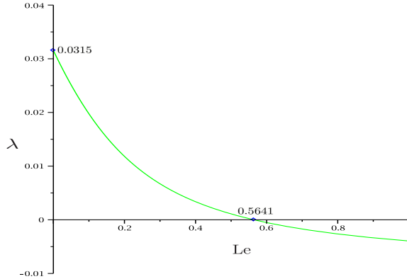
FIGURE 2. Numerical computation of the implicit curve \lambda = \tilde{\varphi}(\text{Le}) for \text{Le} \in (0, \text{Le}_c) , extended beyond \text{Le}_c . Here \theta_i = 0.75 , \ell = 100 , \text{Le}_c \simeq 0.5641 , \lambda_* \simeq 0.0315 . Note that \sqrt{\lambda_1} = \pi/50 \simeq 0.0628 .
