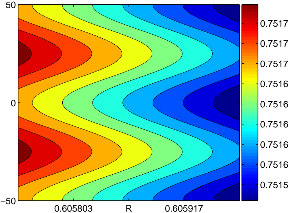
Figure temperature at ignition interface
