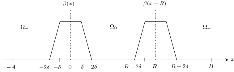
FIGURE 5. Approximation of the mollifier \beta .
