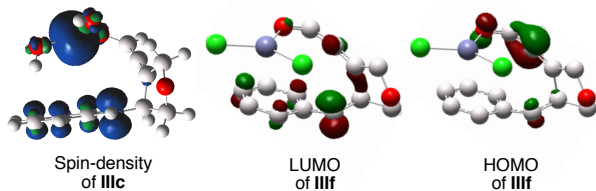
FIGURE 2. Concerted vs step-wise dearomative cyclizations.
