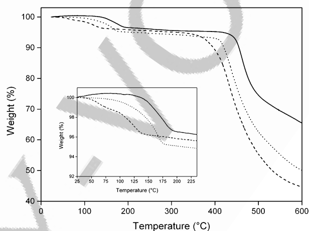
Figure 3. TGA analysis of QxCav (----), MonoTriptyQxCav (.....) and DiTriptyQxCav (—) cavitannds under nitrogen, with enlargement in the inset.
