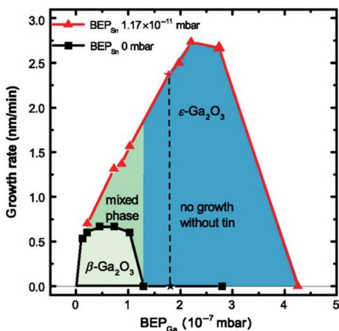
Fig. 6 Comparison of the growth rates as a function of the Ga-flux (expressed as beam equivalent pressure, BEP) during heteroepitaxial growth of Ga 2 O 3 on c -plane sapphire substrates with and without the employment of an additional Sn flux (red triangles and black squares, respectively) via plasma-assisted MBE. The oxygen flow is kept constant at 0.5 standard cubic centimetres per minute with an oxygen plasma power of 150 W. Graph reproduced with permission from ref. 44.
