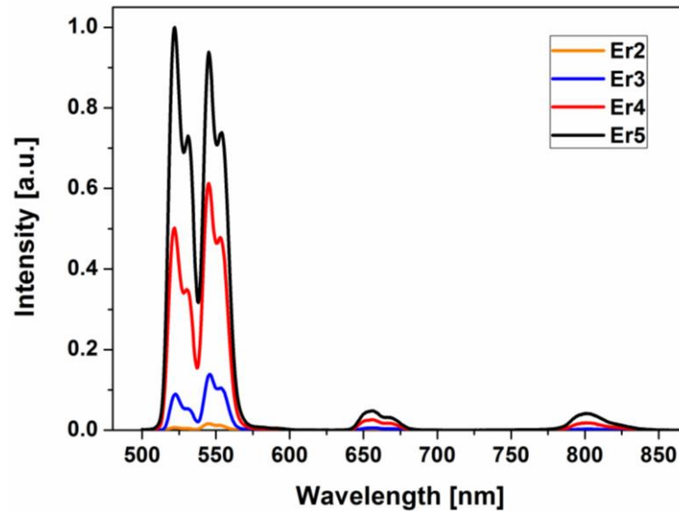
Fig. 5. Emission spectra of the manufactured phosphate glass samples in the wavelength range 500 \div 850 nm obtained under excitation at 976 nm with a CW laser diode. The intensities of the emission are normalized to the green up-conversion band (523 nm) of sample Er5. Visible emission of sample Er1 was too low to be measured.
