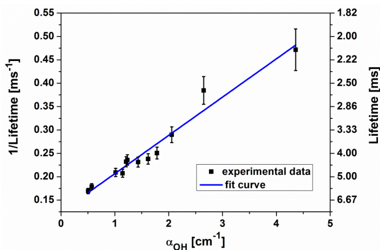
Fig. 1. Decay rate, defined as the inverse of the \text{Er}^{3+}:\text{I}_{13/2} level lifetime, as a function of the absorption coefficient \alpha_{\text{OH}} of \text{OH}^- vibration band at 3000 \text{ cm}^{-1} of all glass samples prepared for the definition of the optimized fabrication process. The experimental data were fitted through the formula (2) reported in Ref. [23]. For the benefit of the reader, measured lifetime values are reported on the right y-axis.
