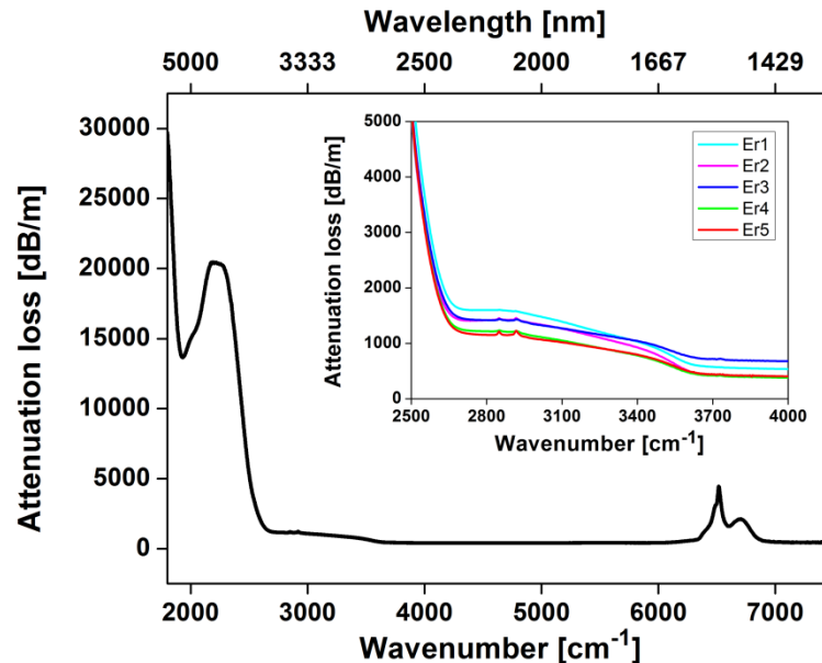
Fig. 3. IR spectrum of glass sample Er5; the inset shows the zoom-up of the \text{OH}^- broad band at 3000\text{ cm}^{-1} of all the manufactured samples Er1 ÷ Er5.
