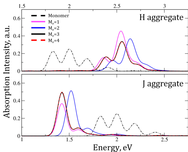
Fig. 2 Absorption spectra calculated for the complete Hamiltonian in Eq.3 only accounting for nearest neighbor interactions. Results are obtained for N=6 , \hbar\omega_0=2.0 eV, \lambda=0.17 eV, \hbar\omega_v=0.17 eV and |J|=0.255 eV. The vibrational basis is truncated setting the maximum number of total vibrational quanta M_v=6 . The electronic basis is truncated fixing the maximum number of excitons M_e to a value ranging from 1 to 4. Results for M_e=1 coincide with those obtained in the HL approximation. Top and bottom panels refer to H-aggregates ( J > 0 ) and J-aggregates ( J < 0 ), respectively.
