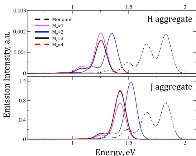
Fig. 3 Emission spectra calculated for the the same system as in Fig. 2. In the upper panel, the monomer emission intensity is rescaled by a factor of 1/400 in order to maintain it comparable to the very weak intensity calculated for the H-aggregate.
