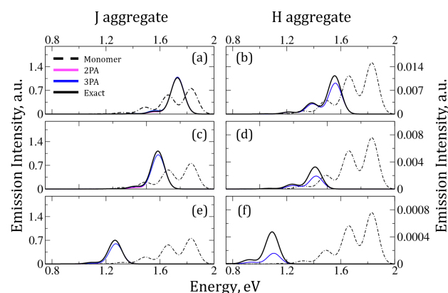
Fig. 8 Emission spectra for 2PA-sp, 3PA-sp and exact excitonic models. Same parameters as in Fig. 7. For H-aggregates (right panels) the intensity of the monomer spectrum is rescaled by a factor 1/50 (panel b), 1/100 (panel d) and 1/1000 (panel f).
