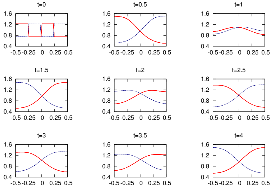
Fig. 7. Evolution of m_h for \nu = 0.12 : solid/red (respectively dashed/blue) lines are used for m_1 , (respectively m_2 ).
