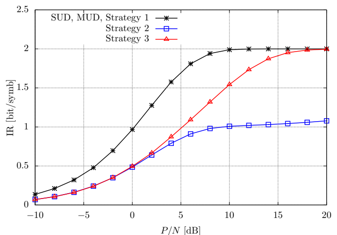
Figure 13: Information rate of "User 1" when it is located at the center of the beam (case 4).
