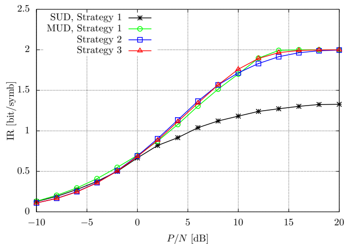
Figure 11: Information rate of "User 1" for case 2.
