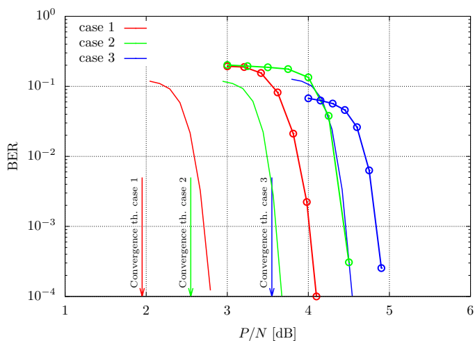
Figure 19: BER curves for “User 1” in the case of strategy 2 for the three interference patterns. Comparison between joint mapping (continuous line) and classical mapping (continuous line with circles).
