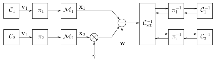
Figure 8: Block diagram of the considered system.
