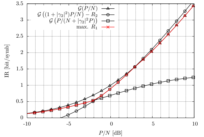
Figure 7: Maximum rate achievable by “User 1”, for K = 2 , Gaussian symbols, and R_2 = 1/2 .
