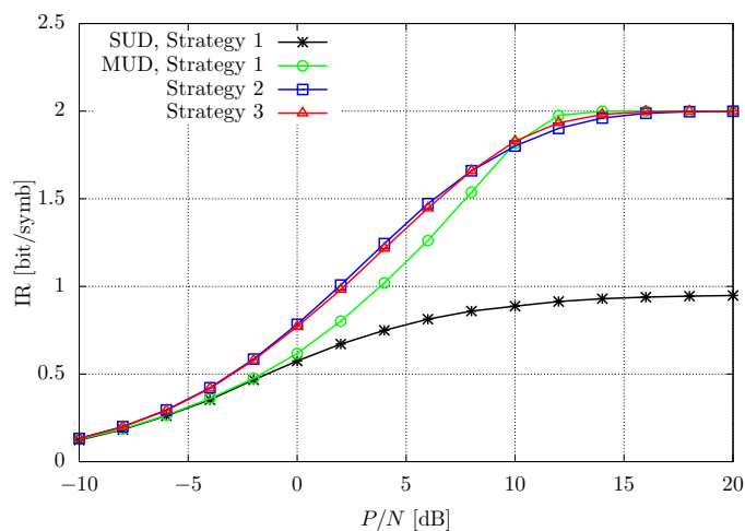
Figure 10: Information rate of "User 1" for case 1.
