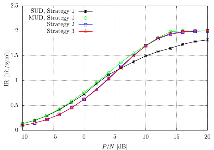
Figure 12: Information rate of "User 1" for case 3.
