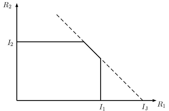
Figure 5: Example of MAC capacity region.
