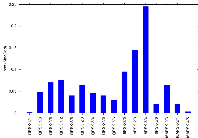
Figure 9: Typical ModCod distribution.
