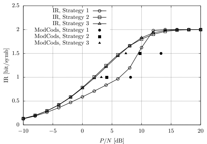
Figure 14: IR and ModCods of “User 1” in case 1. ModCods are based on DVB-S2 LDPC codes.
