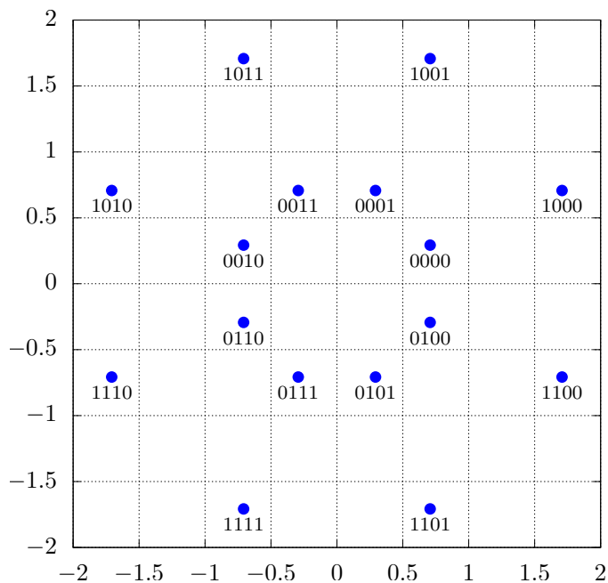
Figure 17: Joint mapping for two QPSK constellations.
