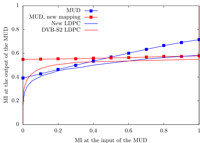
Figure 15: EXIT chart for strategy 2 in case 1 at P/N = 3 dB.
