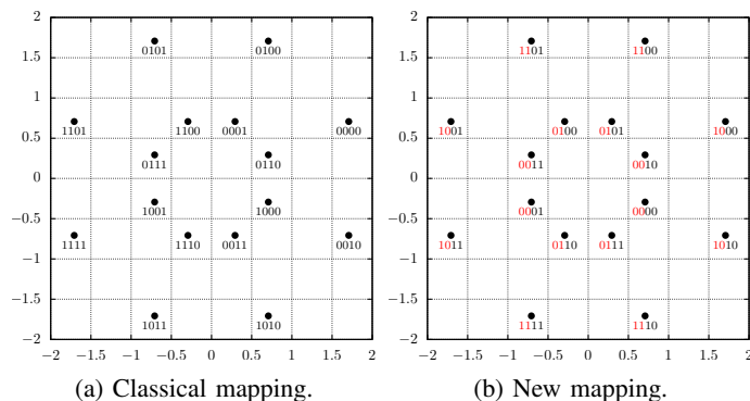
Figure 18: Joint mappings for strategy 1 . Classical (a) and new (b) mapping.
