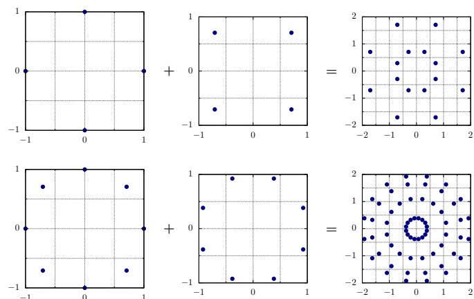
Figure 16: Joint constellations resulting from two QPSK (top) and from two 8PSK (bottom) constellations.
