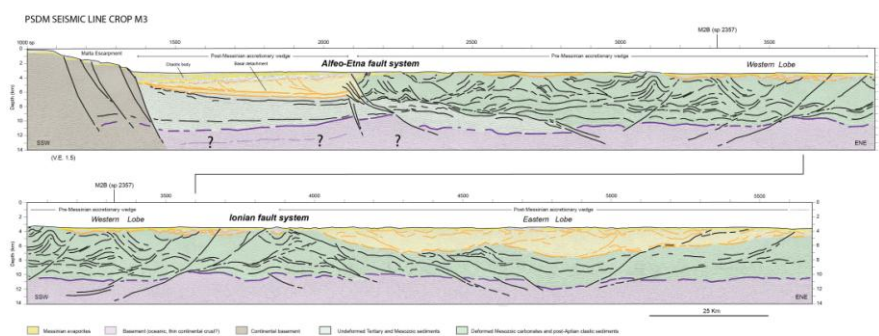
Figure 8 – Pre stack depth migrated MCS line CROP M-3 crossing orthogonally main transverse faults segmenting the subduction system. The seismic line crosses from West to East the Malta escarpment, the WL and EL of the accretionary wedge, which shows different basal detachment depths. The AEF bounds the transition from the salt bearing post-Messinian and the pre-Messinian clastic accretionary wedges in the WL, where a sedimentary basin develops. The IF marks the boundary between the WL and EL and a diffuse area of deformation is observed with displacement of the deep units (i.e. Mesozoic carbonates and basement) accompanied by the formation of a series of ridges and troughs at the seafloor. Major tectono-stratigraphic units are represented by different colors.
