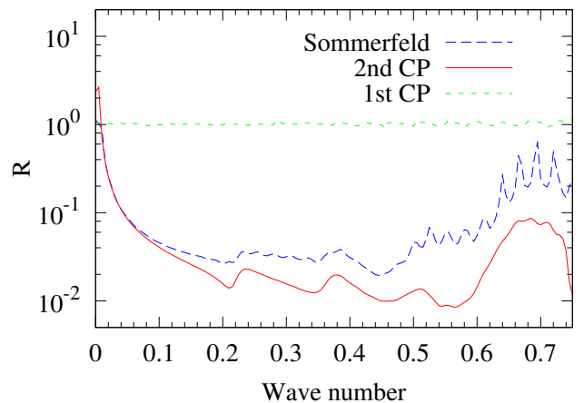
FIG. 3. Experimental reflection coefficient in flat spacetime test. The experimental reflection coefficient, defined in Eq. (103), is plotted versus the wave number for different BCs implemented.
