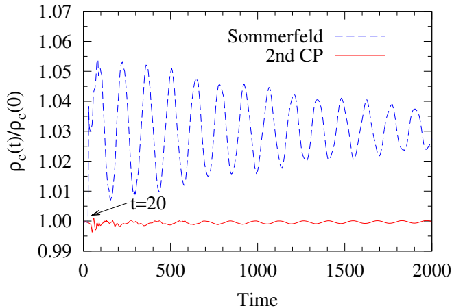
FIG. 1. Radial oscillations of the central rest-mass density of a compact star in time. When Sommerfeld conditions are used a perturbation from the boundary (at r_{\text{out}} = 20 ) hits the center of the star (at t = 20 ) and further perturbs it.
