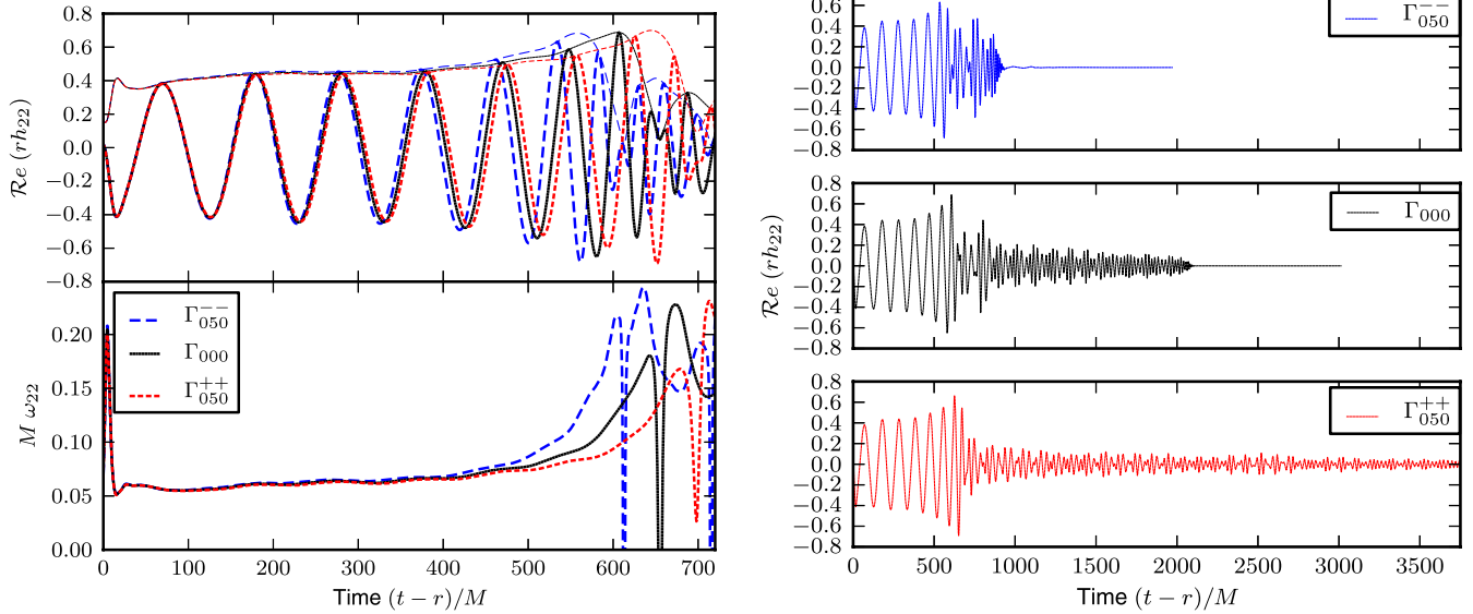
FIG. 8 (color online). Gravitational wave signal for models \Gamma_{050}^{--} , \Gamma_{000} , and \Gamma_{050}^{++} . Left: Inspiral waveforms \Re(rh_{22}) and r|h_{22}| , and frequency M\omega_{22} . Right: Full signal \Re(rh_{22}) .
