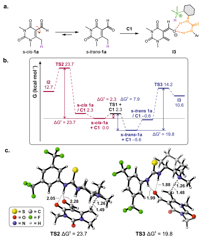
Figure 1. Step 1: Vinylogous dearomative enolization. (a) Overall reaction to dienolate intermediate 13 . (b) Energetic profile of the deprotonation of s-cis 1a (pink) vs s-trans - 1a (blue) by C1 . (c) Transition states (TSs) of the deprotonation of s-cis 1a ( TS2 ) and s-trans 1a ( TS3 ). Energies in kcal·mol -1 , distances in Angstrom (see the Supp. Info for details).
