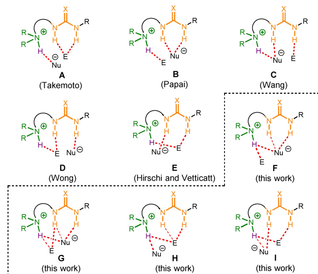
Figure 2. Dual activation modes found operative in the addition of an anionic nucleophile ( Nu - ) to a neutral electrophile ( E ) in the pre-reaction complexes with an amine-thiourea organocatalyst of type C1 . In the dashed box, new activation modes unveiled in this work with the shorter hydrogen-bonds depicted in bold.
