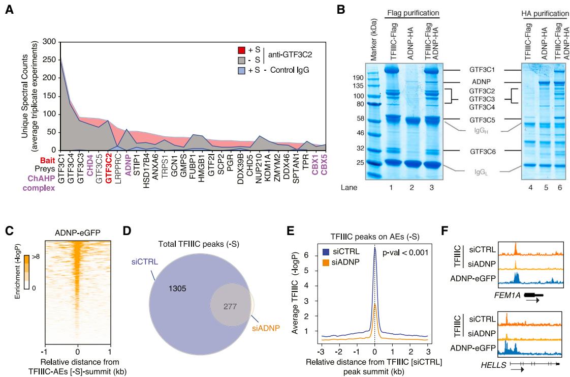
Figure 2. ADNP Guides TFIIIC Selective Recruitment to AEs and TFIIIC-Associated Promoters
