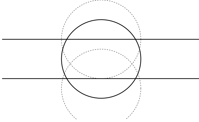
FIGURE 1. The ball in bold line maximizes the volume of the intersection with the slab \Omega .
