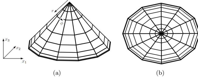
Figure 3: Geometry and graded mesh on a circular cone: viewed from the side (a) and from above (b).
