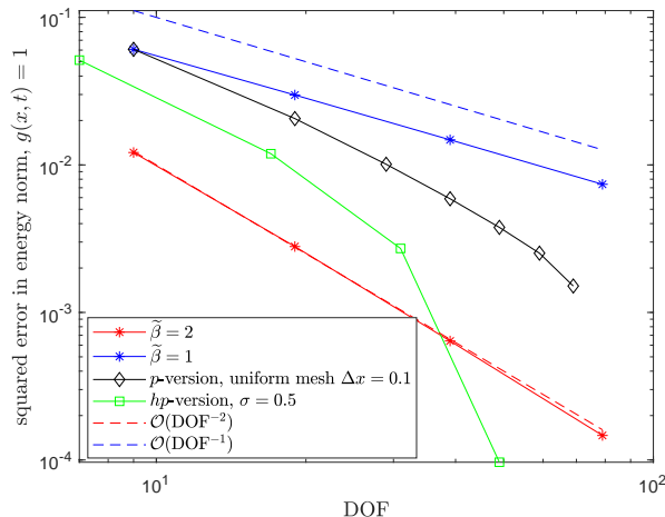
Figure 17: Squared error of the energy norm calculated up to time instant T = 2
