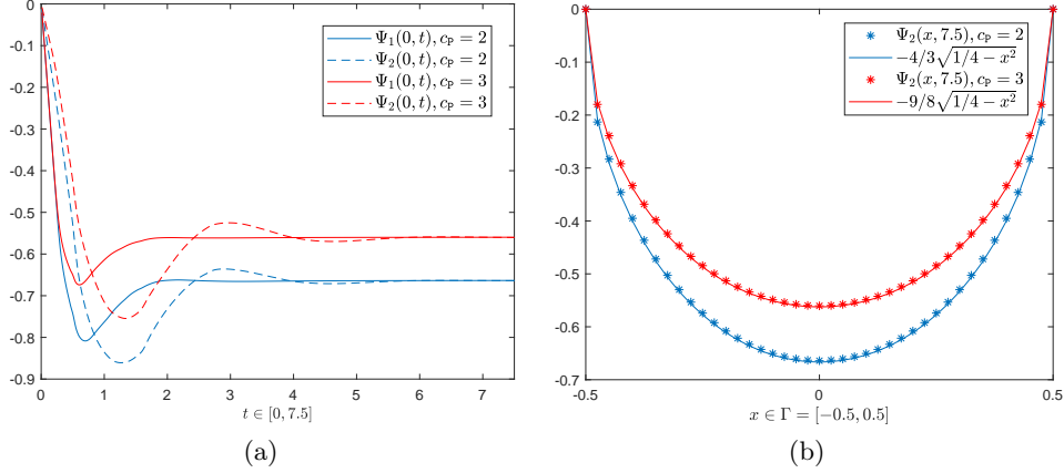
Figure 15: Time history of \Psi_1 and \Psi_2 calculated at the middle point of \Gamma for the couples of velocities c_S = 1, c_P = 2 and c_S = 1, c_P = 3 (a). Vertical component \Psi_2 calculated at the final time instant T = 7.5 and the related elastostatic solution \Psi_{2,\infty}(\mathbf{x}, t) = k_2\sqrt{1/4 - x^2} ( k_2 = -4/3 for c_P = 2 and k_1 = -9/8 for c_P = 3 ) (b).
