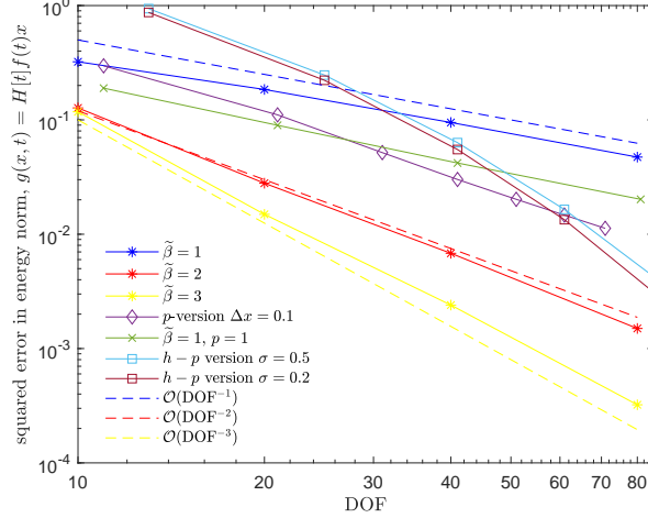
Figure 9: Squared error of the energy norm for various discretization methods
