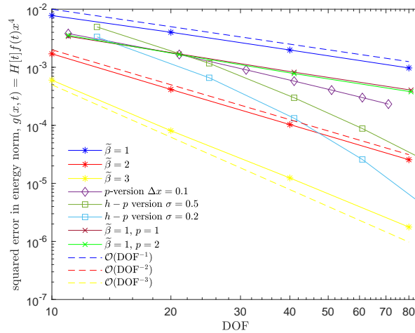
Figure 6: Squared error of the energy norm for various discretization methods.
