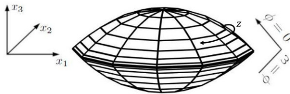
Figure 2: Geometry and graded mesh on the wedge.
