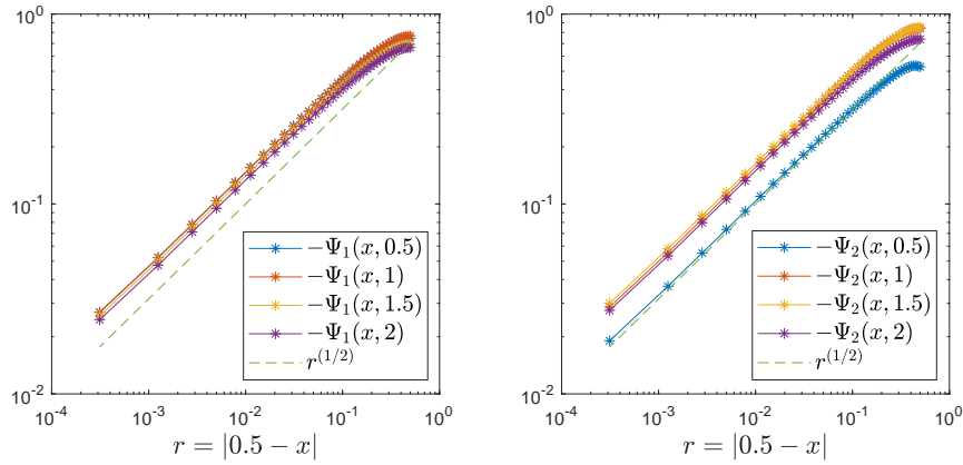
Figure 16: Asymptotic behaviour of -\Psi_1 and -\Psi_2 towards the right end of \Gamma for various time instants ( c_S = 1, c_P = 2 ). The arc is discretized by a \tilde{\beta} -graded mesh with \tilde{\beta} = 2 and 81 mesh points.
