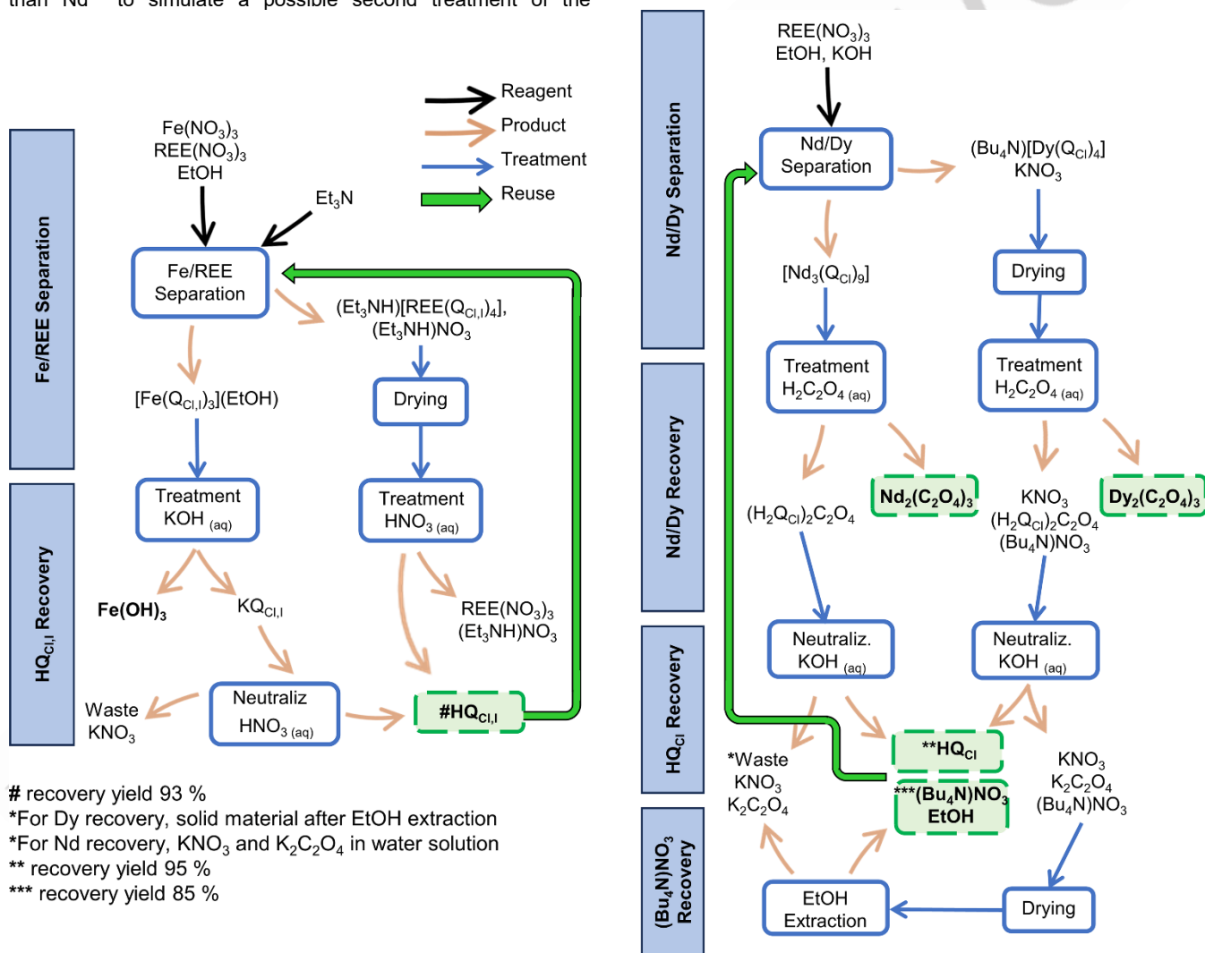
Figure 6. General scheme describing the steps for the sequential separation of the metals from a 1:1:1 Fe 3+ /Nd 3+ /Dy 3+ mixture using HQ Cl /Et 3 N (left) and the separation of Nd 3+ /Dy 3+ from a 1:1 mixture using HQ Cl /KOH/Bu 4 NOH (right) together with the HQ Cl , HQ Cl and Bu 4 N + recovery percentages.
