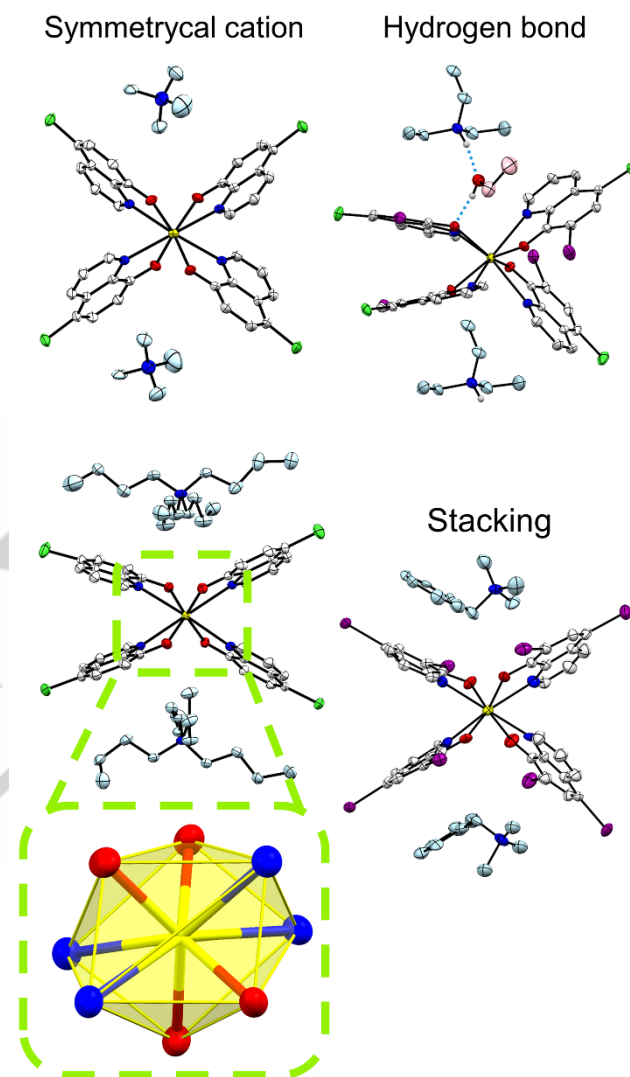
Figure 3. Representation of the different motives in the crystal packings of [Dy(Q R,R ) 4 ] - complexes with different cations. Two cations are shown for every [Dy(Q R,R ) 4 ] - structure, even though the anion:cation ratio in the solid state is 1:1. (Me 4 N)[Dy(Q Cl ) 4 ]-2H 2 O (top left) (Bu 4 N)[Dy(Q Cl ) 4 ]-H 2 O-2EtOH (bottom left), (Et 3 NH)[Dy(Q Cl ) 4 ]-EtOH (top right) and (BnMe 3 N)[Dy(Q I ) 4 ]-0.25THF (bottom right). The coordination around the Dy 3+ ion is highlighted for the structure of (Bu 4 N)[Dy(Q Cl ) 4 ]-H 2 O-2EtOH. Hydrogen bonds between Et 3 NH + , EtOH and the complex in the structure of (Et 3 NH)[Dy(Q Cl ) 4 ]-EtOH are shown as dotted lines. Atom colors: O, red; N, blue; C, grey (complex)/light blue (cation)/pink (solvent); Dy, yellow; Cl, green; I, purple.
