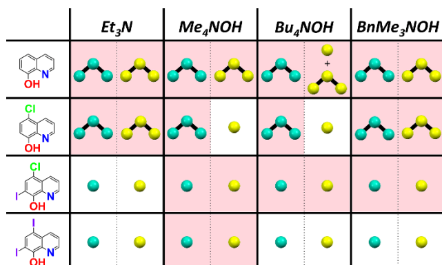
Figure 2. Visual representation of the synthetic conditions used for the preparation of REE-complexes (hydroxyquinoline in row, base in column) and corresponding isolated complexes (● = tetrakis complex for REEs; ●-●-● = trinuclear complex). White and light red backgrounds highlight the conditions in which the complexes are soluble or not completely soluble, respectively, in the reaction environment. For syntheses performed with the same ligand and base, the reactions were performed with the same concentration of Nd 3+ and Dy 3+ (range 5-25 mM). Cyan, Nd; Yellow, Dy
