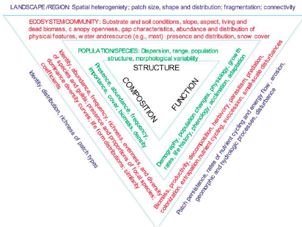
Figure 4. Triangular representation of the ecological hierarchy, with the most important characteristics of the concepts of composition, structure and function (Source Dale & Beyeler: from Franklin 1988 and Noss 1990).
