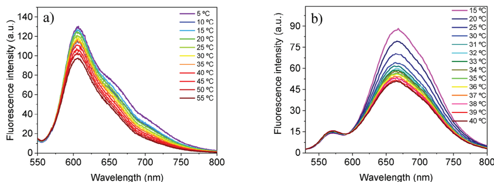
Figure 1. Emission spectra at different temperatures of water suspensions of ONPs containing a 26% in mol of radical for a) PTM-d-ONPs excited at \lambda_{\text{exc}} 385 nm and b) TTM-d-ONP excited at \lambda_{\text{exc}} 377 nm. 13e
