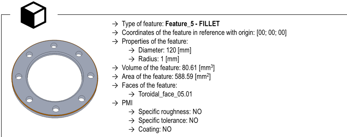
Figure 7: examples of geometric features recognized for a flange 3D model
