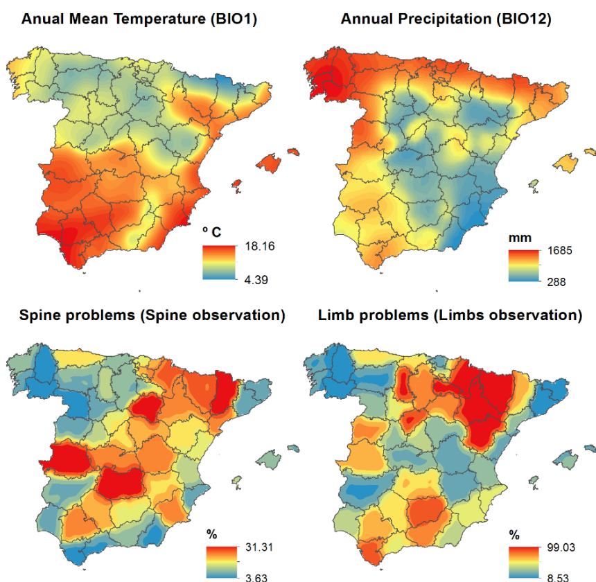
Figure 3 – Distribution maps for annual mean temperature (°C), annual rainfall (mm), and spine and limb observation variables using rate data between 2012 and 2016 interpolated by Ordinary Kriging.
