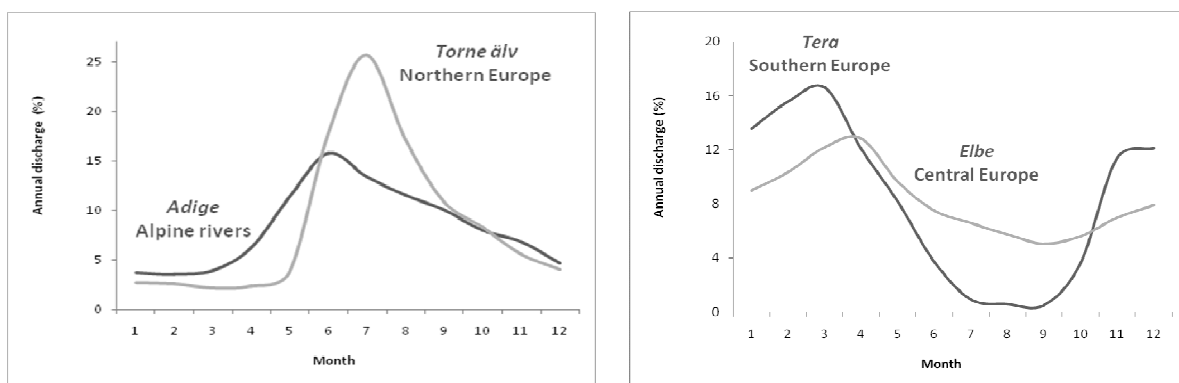
Fig. 2.2- Hydrological regime of four European rivers: Torne älv (Sweden), Adige (Italy), Tera (Spain) and Elbe (Central Europe)
