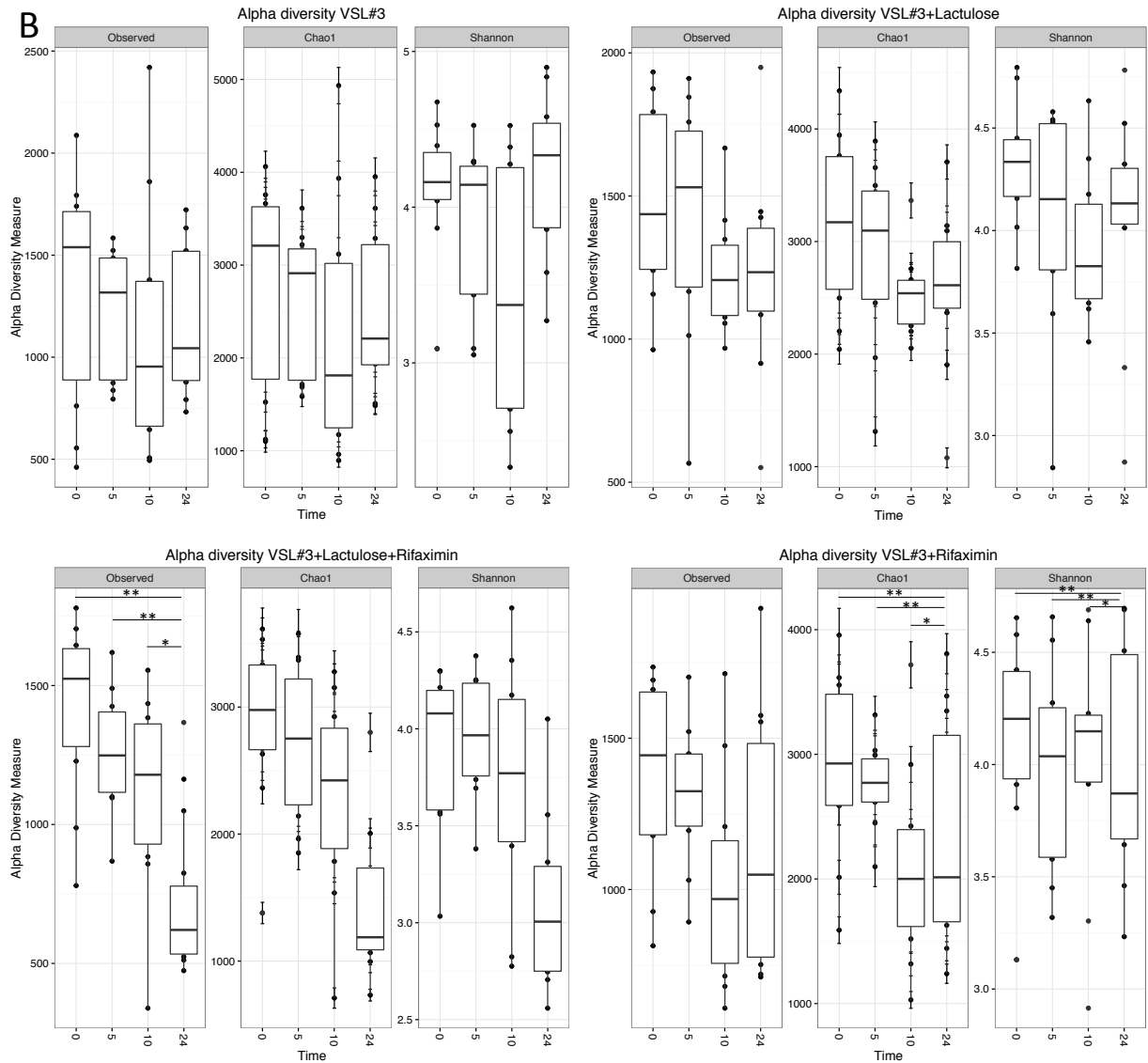
Figure 2B. Measure of bacterial diversity. Alpha-diversity calculated on the number of observed OTUs, the Chao1 index and the Shannon entropy index, for CP subjects, overtime for each condition considered: VSL#3, VSL#3+Lactulose, VSL#3+Lactulose+Rifaximin, VSL#3+Rifaximin. *p-value \leq 0.05, **p-value \leq 0.01. The body of the box plot represents the first and third quartiles of the distribution and the median. The whiskers extend from the quartiles to the last datapoint within 1.5 \times IQR with outliers beyond represented as dots.
