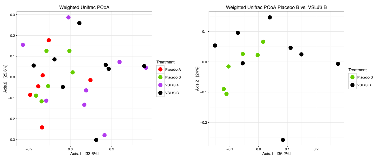
Figure 3. PCoA plots of bacterial beta-diversity based on the Weighted UniFrac distance according to groups of treatments ( left ) and groups of treatments after the 3 month-therapy ( right ). Placebo A, placebo at baseline; placebo B, placebo at 3 months; VSL#3 A, VSL#3 at baseline; VSL#3 B, VSL#3 at 3 months.
