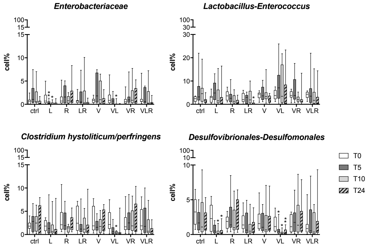
Figure 6B. Bacteria cells enumeration through FISH/FCM, at times 0, 5, 10, and 24 (median-max/min, N = 10) for CP subjects. *p-value \leq 0.05 , **p-value \leq 0.01 , ***p-value \leq 0.001 , paired t-test, treatment vs ctrl. ctrl, control; L, Lactulose; R, rifaximin; LR, Lactulose + Rifaximin; V, VSL#3; VL, VSL#3+Lactulose; VR, VSL#3+Rifaximin; VLR, VSL#3 + lactulose + rifaximin. For the different FISH tested, percentage of positive cells were calculated on gated total bacterial cells.
