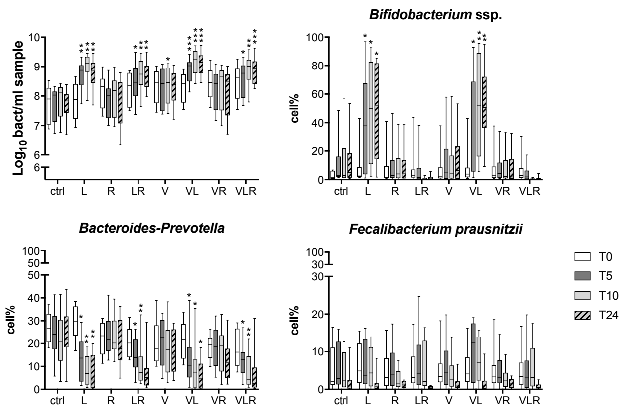
Figure 6A. Bacteria cells enumeration through FISH/FCM, at times 0, 5, 10, and 24 (median-max/min, N = 10) for CP subjects. *p-value \leq 0.05 , **p-value \leq 0.01 , ***p-value \leq 0.001 , paired t-test, treatment vs ctrl. ctrl, control; L, Lactulose; R, rifaximin; LR, Lactulose + Rifaximin; V, VSL#3; VL, VSL#3+Lactulose; VR, VSL#3+Rifaximin; VLR, VSL#3 + lactulose + rifaximin. For the different FISH tested, percentage of positive cells were calculated on gated total bacterial cells.
