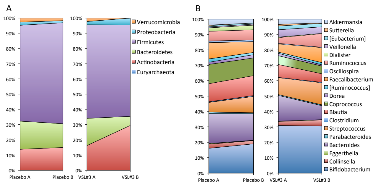
Figure 4. Relative abundance of microbial taxa at phylum (A) and genus (B) level. Only taxa with abundance > 0.001 are depicted. Placebo A, placebo at baseline; placebo B, placebo at 3 months; VSL#3 A, VSL#3 at baseline; VSL#3 B, VSL#3 at 3 months.
