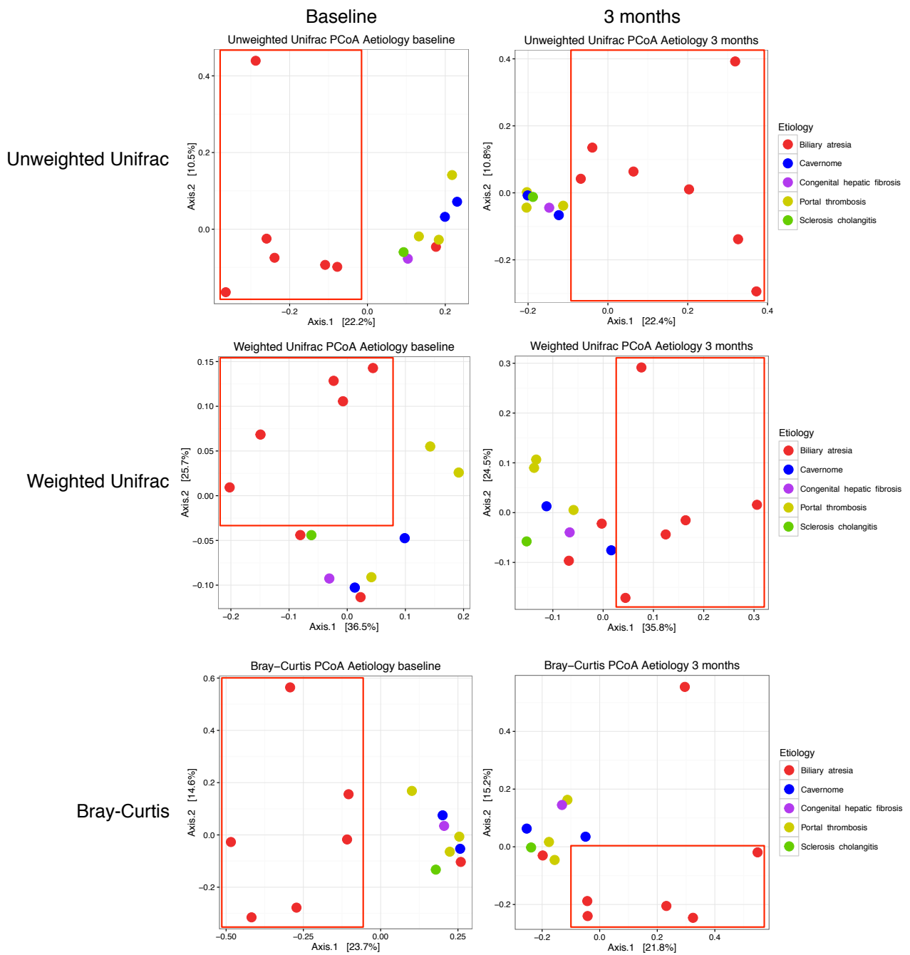
Figure S2. Measures of bacterial diversity. PCoA plots of bacterial beta-diversity based on Unweighted and Weighted UniFrac distances and the Bray-Curtis dissimilarity analyzed according to aetiologies.
