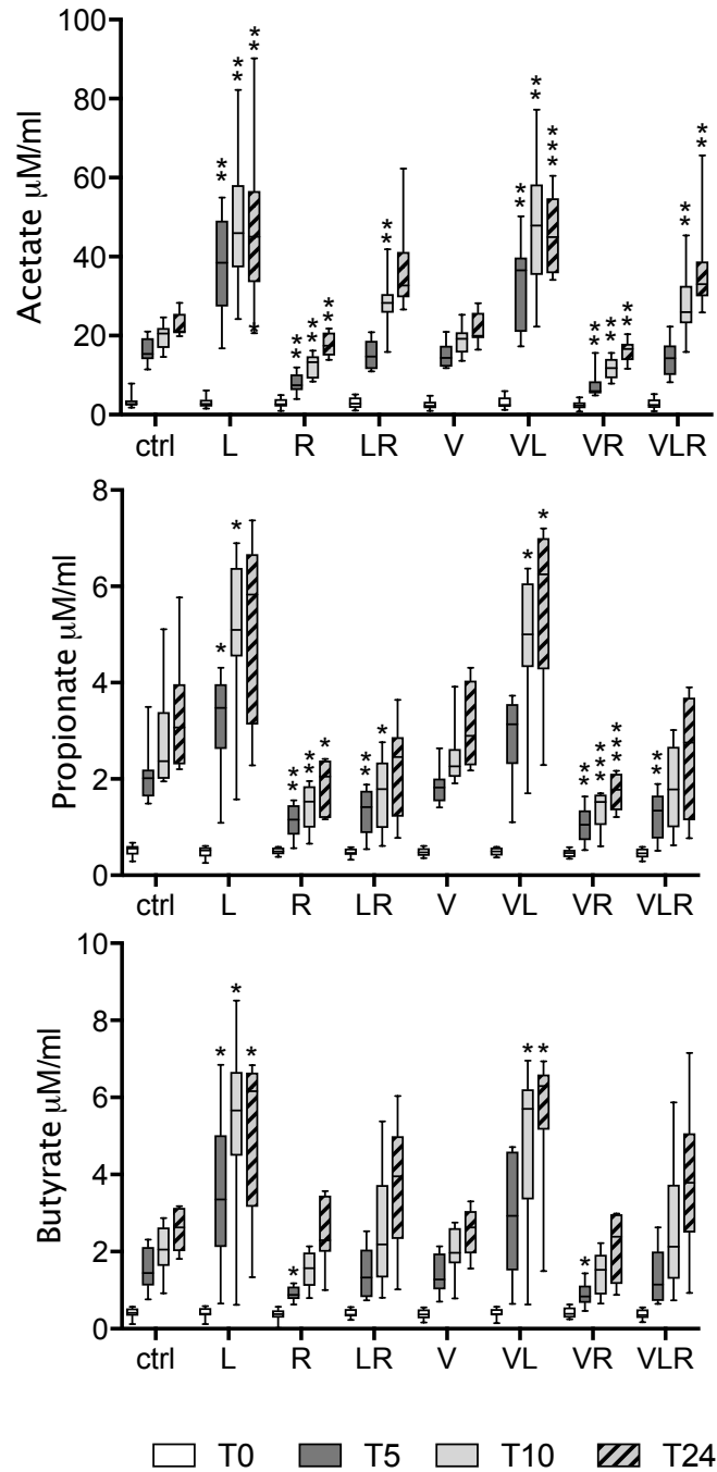
Figure 8. SFGA production at times 0, 5, 10, 24 for Acetate, Propionate and Butyrate (median-max/min, N = 10) in CP subjects. *p-value \leq 0.05, **p-value \leq 0.01, ***p-value \leq 0.001, paired t-test, treatment vs ctrl. ctrl, control; L, Lactulose; R, rifaximin; LR, Lactulose + Rifaximin; V, VSL#3; VL, VSL#3+Lactulose; VR, VSL#3+Rifaximin; VLR, VSL#3 + lactulose + rifaximin.
