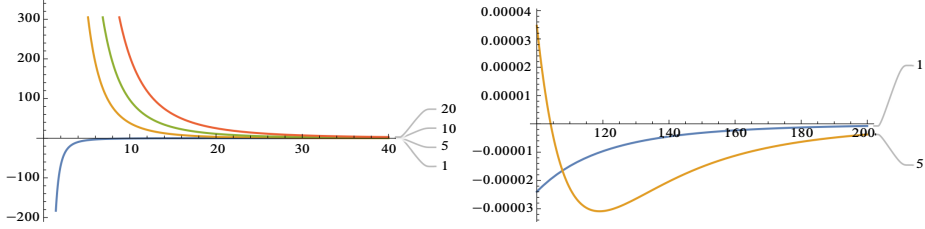
Figure 2. Plot of \mathcal{S}_0^k versus T for k = 1, 5, 10, 20 . On the right, same with k = 1 and 5 which shows the intersection of the two curves at large enough T .
