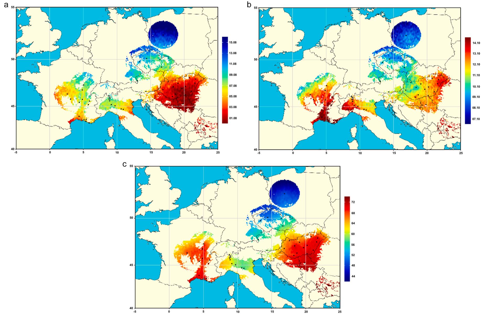
Fig. 4. Mean start date (a), mean end date (b), and mean duration (days) (c) of the ragweed pollen season for Europe, with the geographical locations of the aerobiological stations, using the raw data sets, 16 years, 1995–2010. The stations (1) with mean annual pollen concentration smaller than 100 \text{ pollen grains} \cdot \text{m}^{-3} of air, as well as (2) the areas beyond \pm 100 \text{ m} from the altitude of the stations within their 150 km radius are excluded from mapping, and (3) the maximum distance is 150 km to each station. Horizontal axis: longitude, angle in degrees; vertical axis: latitude, angle in degrees. Locations of the aerobiological stations are indicated by black dots.
