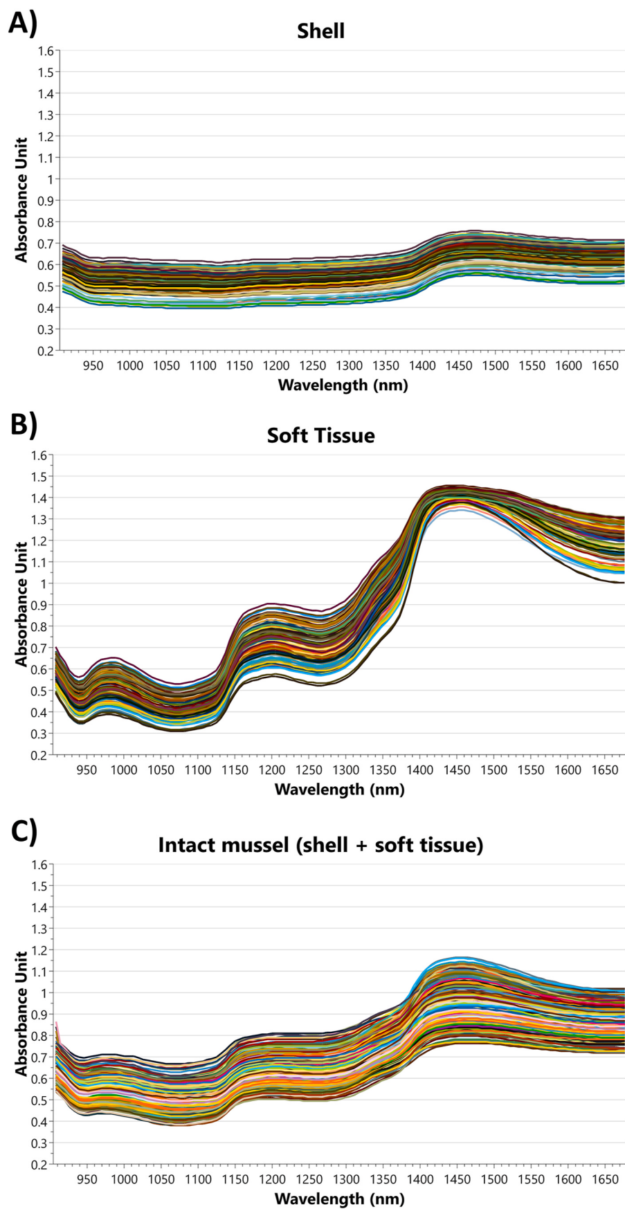
Fig. 3. Comparison among raw absorbance ( \log_{10}1/R ) NIR spectra (908–1676 nm) of representative samples of mussel shells (A), mussel soft tissues (B) and intact mussels (shells + soft tissues) (C).
