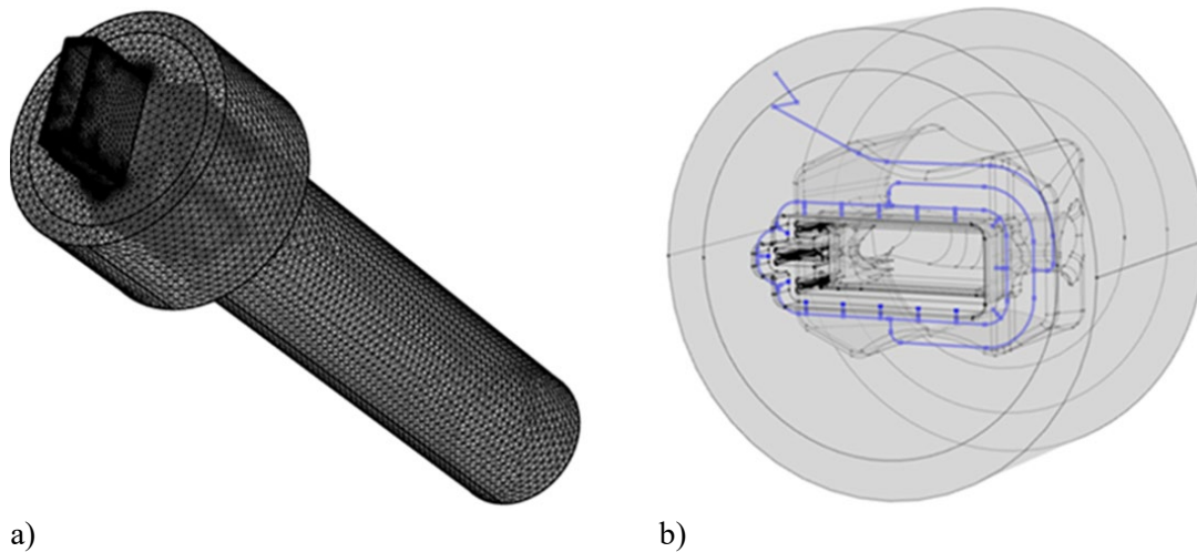
Fig.8 The geometrical model for the simulation tests: a) the billet and the die set for uncooled process, b) the tooling set combined with the 1D cooling channel
