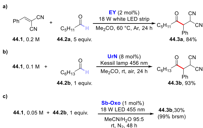
Scheme 44. Hydroacylation of Benzylidene Malononitrile Triggered by Different PC S HAT
