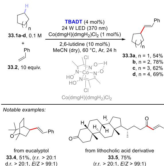
Scheme 33. Dual-Catalyzed Dehydrogenative (E)-Alkenylation of Cycloalkanes
