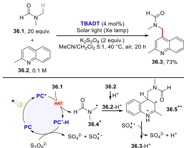
Scheme 36. Photocatalyzed Cross-Dehydrogenative Coupling between Amides and Heteroarenes
