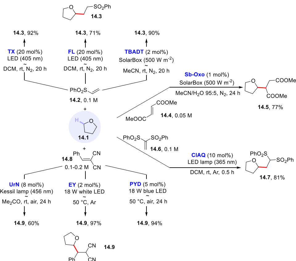
Scheme 14. Different PC S HAT for the Photocatalyzed Cleavage of the C–H Bond in THF
