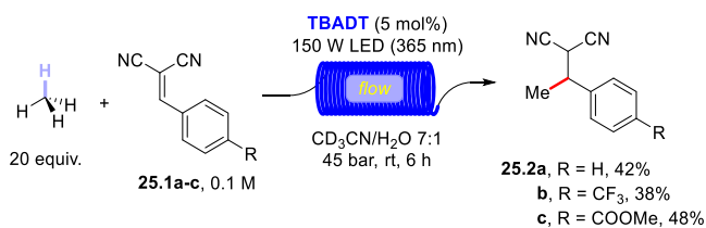
Scheme 25. Photocatalyzed Derivatization of Methane under Flow Conditions
