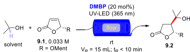
Scheme 9. Photocatalyzed Functionalization of Furanones under Flow Conditions
