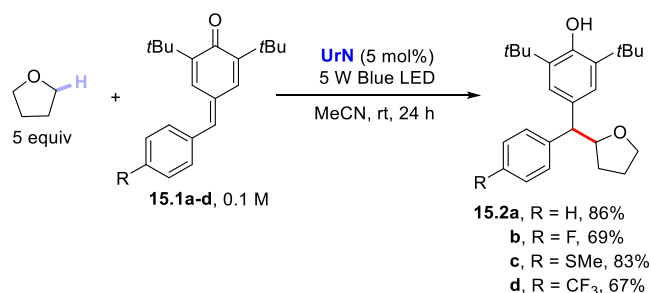
Scheme 15. Photocatalyzed Addition of THF onto Cyclohexa-2,5-dien-1-ones
