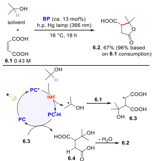
Scheme 6. Photoaddition of Isopropanol onto Maleic Acid
