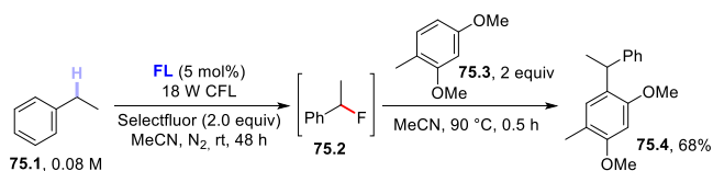
Scheme 75. One-Pot Arylation of Unactivated Benzylic C–H Bonds
