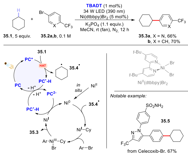
Scheme 35. Arylation of Strong C–H Bonds via a TBADT/ Nickel Dual-Catalyzed Strategy
