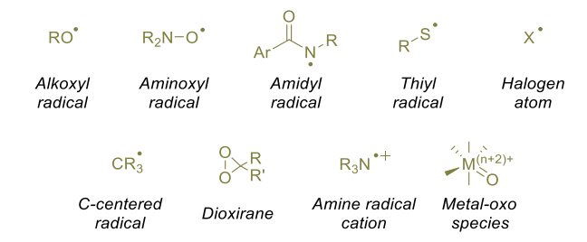
Scheme 4. Common Hydrogen Abstractors Used in Synthetic Planning
