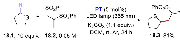
Scheme 18. Allylation of Tetrahydrothiophene
