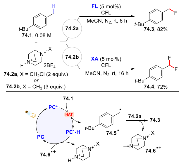
Scheme 74. Diarylketone-Photocatalyzed Selective Benzylic Mono- and Difluorinations
