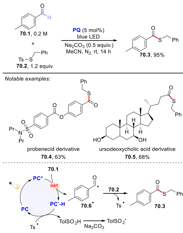
Scheme 70. Photocatalyzed Thioesterification of Aldehydes
