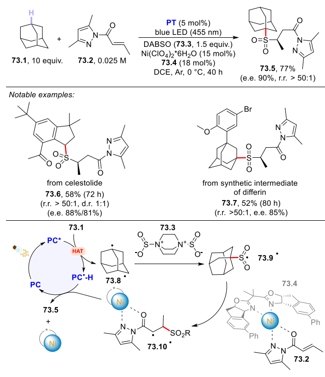
Scheme 73. Three-Component Asymmetric Sulfonation via HAT
