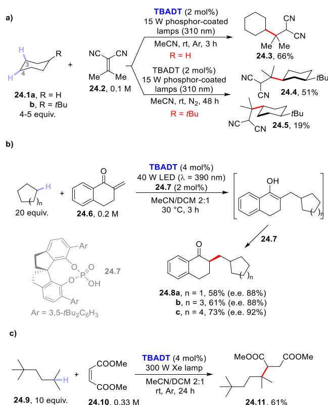
Scheme 24. Photocatalyzed C-H Cleavage in (Cyclo)alkanes
