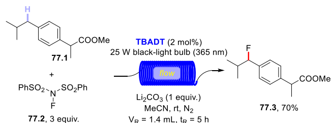
Scheme 77. TBADT-Photocatalyzed Benzylic Fluorination in Flow
