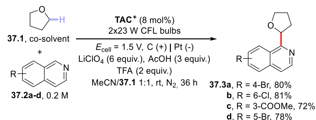
Scheme 37. Electrophotocatalytic Arylation of Ethers Mediated by the Trisaminocyclopropenium (TAC + ) Ion
