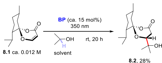
Scheme 8. Photocatalyzed Synthesis of 1,5-Dioxaspiro[5.5]undecane-2-ones
