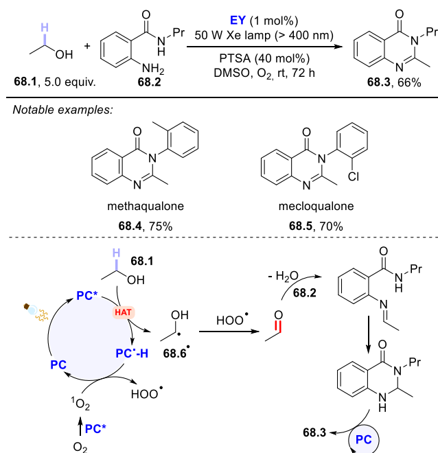
Scheme 68. EY-Photocatalyzed Synthesis of Alkyl Quinazolinones via Oxidation of Primary Alcohols
