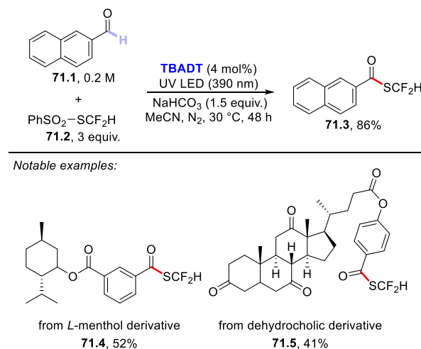
Scheme 71. Difluoromethylthiolation of Aldehydes
