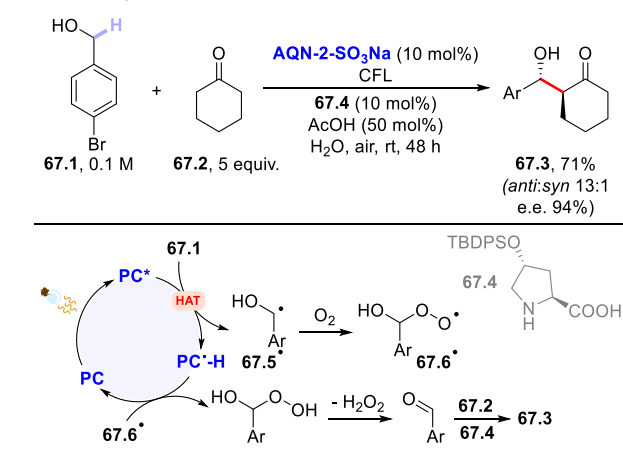
Scheme 67. One-Pot Asymmetric Aldol Reaction Starting from Benzyl Alcohols under Aerobic Conditions
