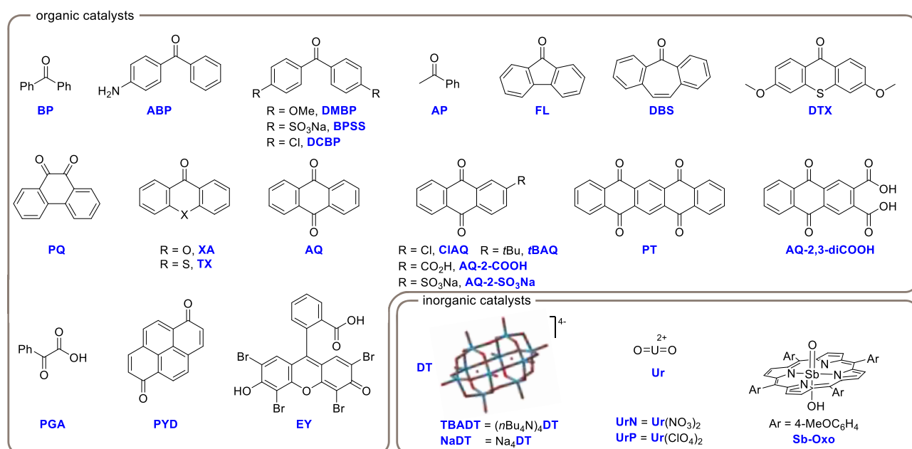
Figure 1. Main photocatalysts (PCs HAT ) used in photocatalyzed HAT: BP, benzophenone; ABP, aminobenzophenone; DMBP, 4,4'-dimethoxybenzophenone; BPSS, disodium benzophenonedisulfonate; DCBP, 4,4'-dichlorobenzophenone; AP, acetophenone; FL, 9-fluorenone; DBS, dibenzosuberone; DTX, 3,6-dimethoxy-9H-thioxanthen-9-one; PQ, 9,10-phenanthrenequinone; XA, xanthone; TX, thioxanthone; AQ, anthraquinone; CIAQ, 2-chloroanthraquinone; tBAQ, 2- tert -butylanthraquinone; AQ-2-COOH, anthraquinone-2-carboxylic acid; AQ-2-SO 3 Na, anthraquinone-2-sulfonic acid sodium salt; PT, 5,7,12,14-pentacenetetrone; AQ-2,3-diCOOH, anthraquinone-2,3-dicarboxylic acid; PGA, phenylglyoxylic acid; PYD, 1,6-pyrenedione; EY, Eosin Y; DT, decatungstate anion (TBADT, tetrabutylammonium decatungstate; NaDT, sodium decatungstate); Ur, uranyl cation (UrN, uranyl nitrate hexahydrate; UrP, uranyl perchlorate); Sb-Oxo, antimony-oxo tetra-( p -methoxyphenyl)-porphyrin.
