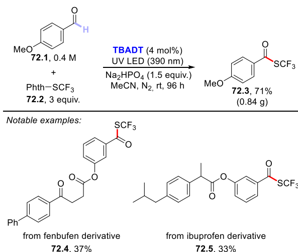
Scheme 72. Trifluoromethylthiolation of Aldehydes
