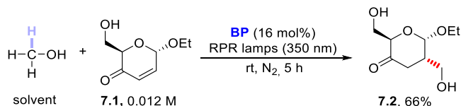
Scheme 7. Photocatalyzed Functionalization of an \alpha -Enone
