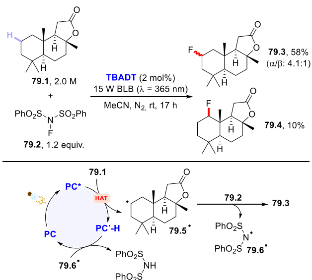
Scheme 79. Photocatalytic Fluorination of Unactivated C–H Bonds
