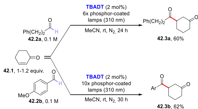
Scheme 42. Cyclohexenone Acylation by Addition of Aliphatic (Upper Part) and Aromatic (Lower Part) Aldehydes
