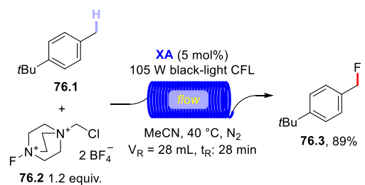
Scheme 76. Photocatalyzed Benzylic Fluorination under Flow Conditions
