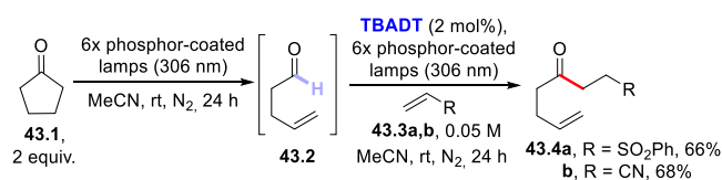
Scheme 43. Preparation of Homoallyl Ketones from Cyclopentanones via a Two-Step Photochemical Norrish Type-I Cleavage/Photocatalyzed Hydroacylation Sequence
