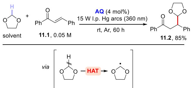
Scheme 11. Photocatalyzed Incorporation of a Masked Formyl Group
