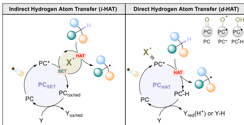
Scheme 5. Photocatalyzed Indirect Hydrogen Atom Transfer ( i -HAT) vs Direct Hydrogen Atom Transfer ( d -HAT)
