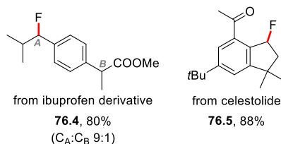
Scheme 77. TBADT-Photocatalyzed Benzylic Fluorination in Flow
