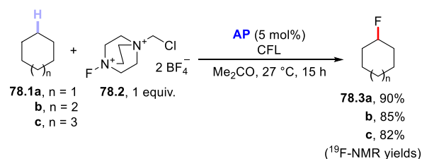
Scheme 79. Photocatalytic Fluorination of Unactivated C–H Bonds
