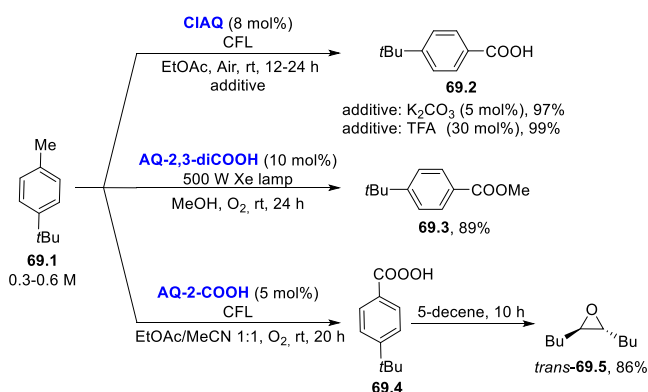
Scheme 69. Anthraquinone-Photocatalyzed Benzylic Oxidation of Methylarenes
