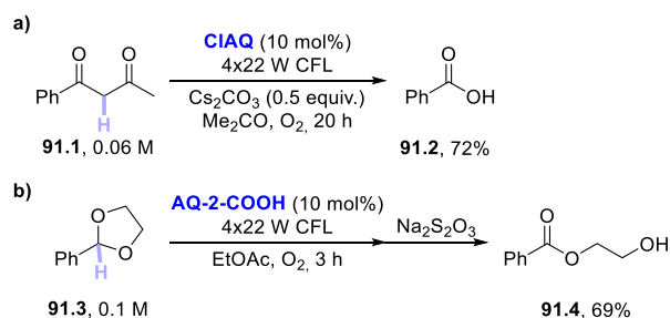
Scheme 91. Aerobic Photooxidative Cleavage of (a) 1,3-Diketones and (b) 1,3-Dioxolanes
