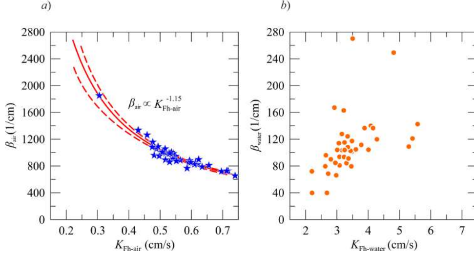
Figure 4: Correlation between \beta and K_{Fh} a) for air, and b) for water. Symbols refer to experimental data, the bold curve refers to the interpolating power function, dashed curves refer to 95% confidence limits.
