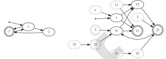
Fig. 4. Graph and its corresponding extension for k = 2 .
