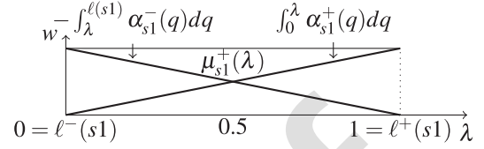
Fig. 2. Computation of \ell^+(s1) = 1 and \ell^-(s1) = 0 .
