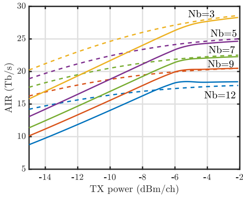
Figure 4. AIR (Tb/s) vs. P_c (dBm) for blocks of length [3, 5, 7, 9, 12] spans, 40 WDM CIP channels, pump P_p = 25\text{mW} , span loss A = 16.5\text{dB} , EDFA length \ell = 8.3\text{m} . no NLI. Solid: GFF with excess loss 0.3dB; dashed: no-GFF.
