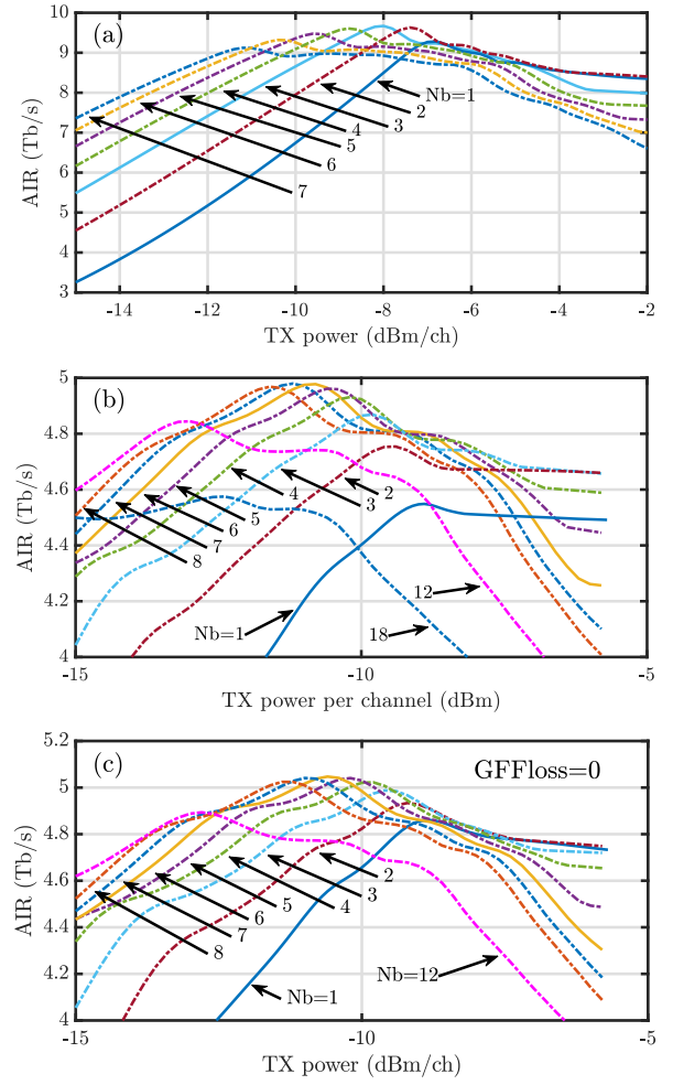
Figure 7. AIR vs. P_c for transmission of 40 WDM CIP channels over 287 spans, span loss A = 9.5 dB, EDFA length \ell = 5.3 m, at various sparse-GFF block sizes N_b . (a) P_p = 25 mW, GFF loss 0.3dB (b) P_p = 11 mW, GFF loss 0.3dB; (c) P_p = 11 mW, zero GFF loss. NLI included.
