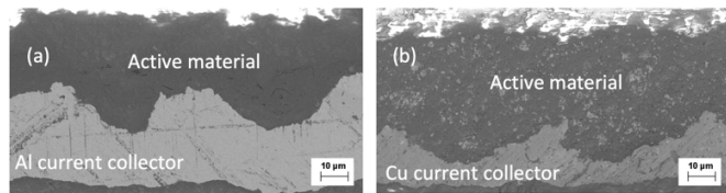
Figure 5. SEM images of electrode sections for complete: (a) cathode and (b) anode with textured current collectors.
