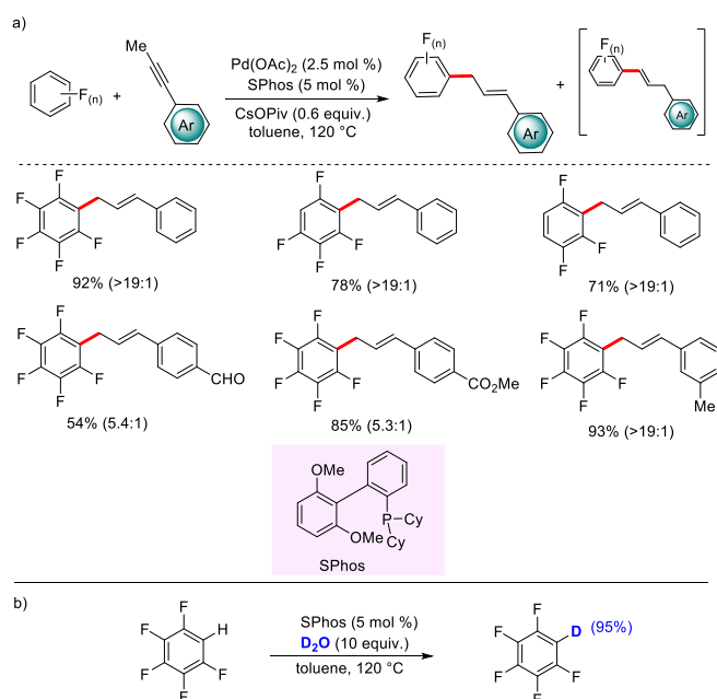
polyfluoroarenes with alkynes (a); H/D exchange experiment (b).
