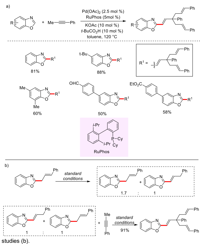
Scheme 11. Palladium/acid-catalyzed C–H trisallylation of azoles (a); Mechanistic
