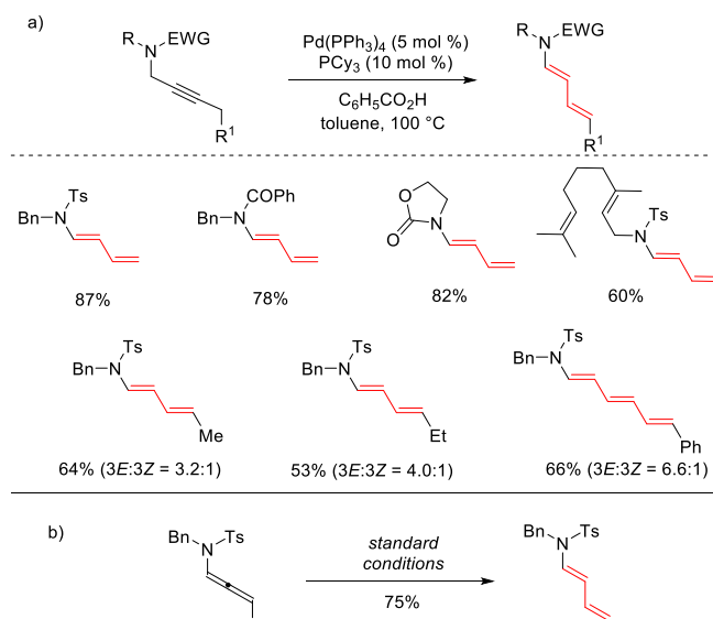
Scheme 16. Bi-directional alkyne isomerization via Pd(0)/carboxylic acid catalysis: expedient access to 1,3-dienes (a); Control experiment with allenamide intermediate (b).
