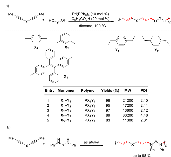
Scheme 21. Pd/benzoic acid-catalyzed regio- and stereoselective polymerization of internal diynes and diols.
