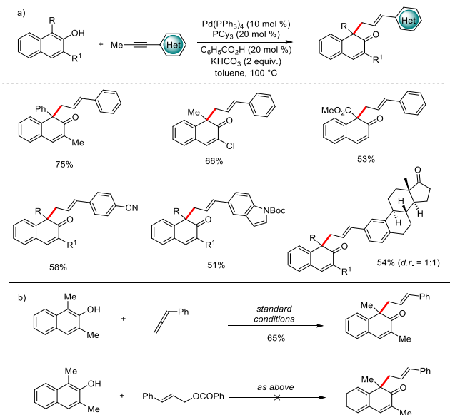
Scheme 4. Redox-neutral Pd(0)-catalyzed dearomatization of \beta -naphthols with alkynes (a); Mechanistic studies (b).
