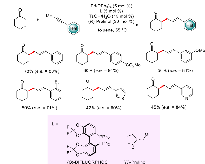
Scheme 31. Enantioselective, palladium-catalyzed \alpha -allylation of ketones with
