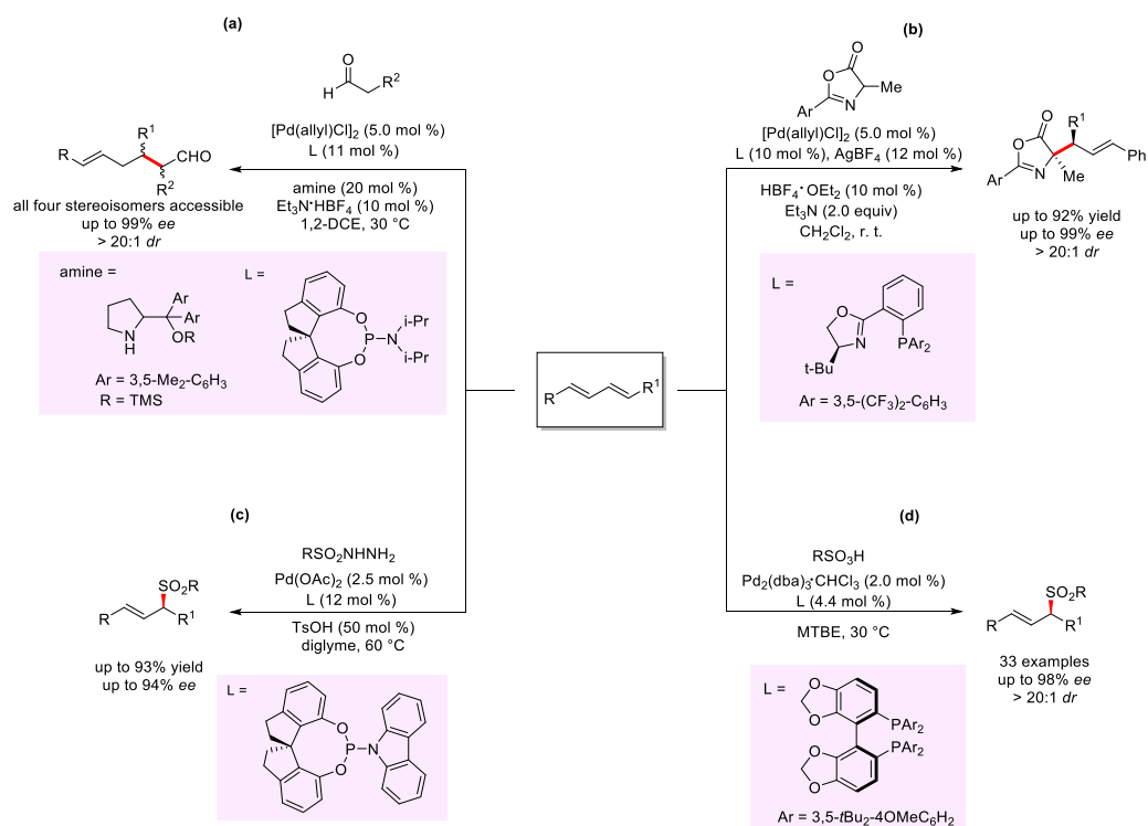
Scheme 34. Enantioselective, palladium/Brønsted acid-catalyzed, Tsuji-Trost functionalizations using 1,3-dienes.
