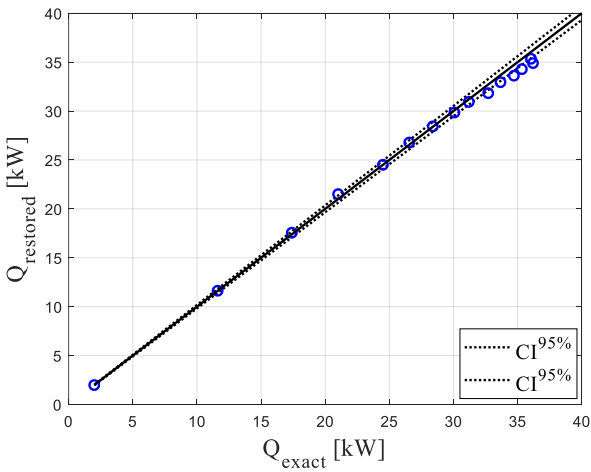
Figure 5. Correlation between the estimated and exact heat transfer rates for Re_s=18'370
