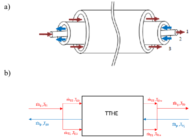
Figure 1. TTHE under investigation. a) 3D representation; b) system schema.
