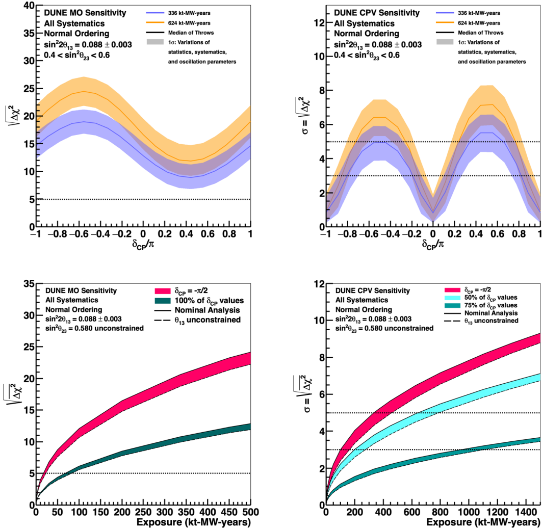
FIG. 3. Sensitivity to the neutrino mass ordering (left) and CP violation (right) as a function of the true value of \delta_{CP} for several exposures (top) or as a function of exposure in kt-MW-years (bottom), with the Phase II near detector. For the top plots, the solid line shows the median sensitivity while the width of the band represents 68% of variations of statistics, systematics, and oscillation parameters. In the bottom plots, only the Asimov sensitivity is considered and the width of the bands represents the difference between the nominal analysis, which uses the external constraint from reactor antineutrino experiments on \sin^2\theta_{13} , and an analysis without this constraint. Curves are shown for maximal CP violation ( \delta_{CP} = -\pi/2 ) and for different fractions of \delta_{CP} values.
