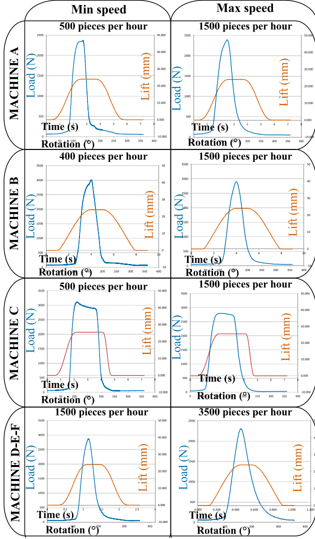
Fig. 12: Experimental load and lift graphs of the compression slide that moves according to polynomial law during Cork_02 insertion.
