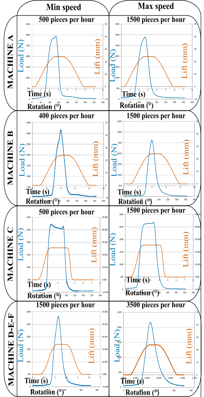
Fig. 14: Experimental load and lift graphs of the compression slide that moves according to polynomial law during Cork_03 insertion.
