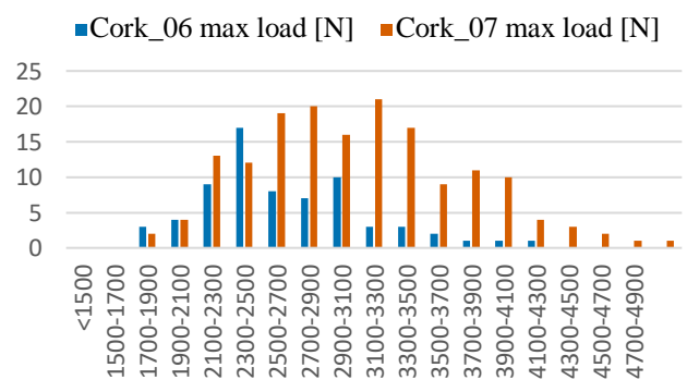
Fig20: Frequency graph on maximum load detected during 100 insertions of Cork_06 and 100 insertions of Cork_07
