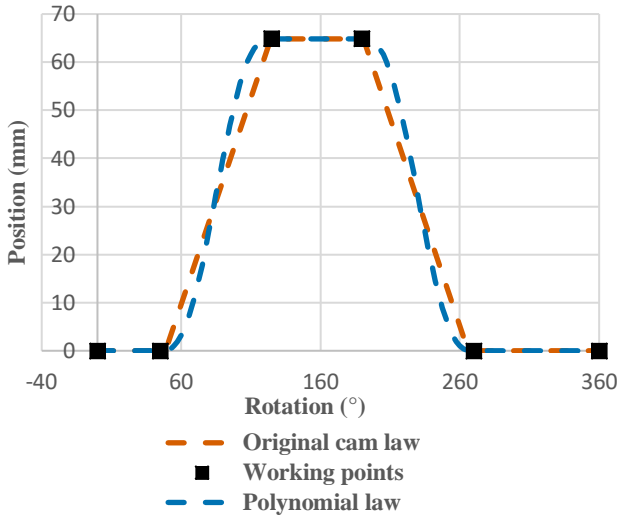
Fig. 3: the law of motion imposed by the cam of the bottle tray cylinder in the MACHINE-A.
