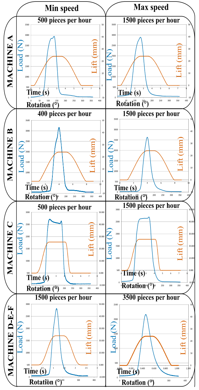
Fig. 14: Experimental load and lift graphs of the compression slide that moves according to polynomial law during Cork_03 cap insertion.
