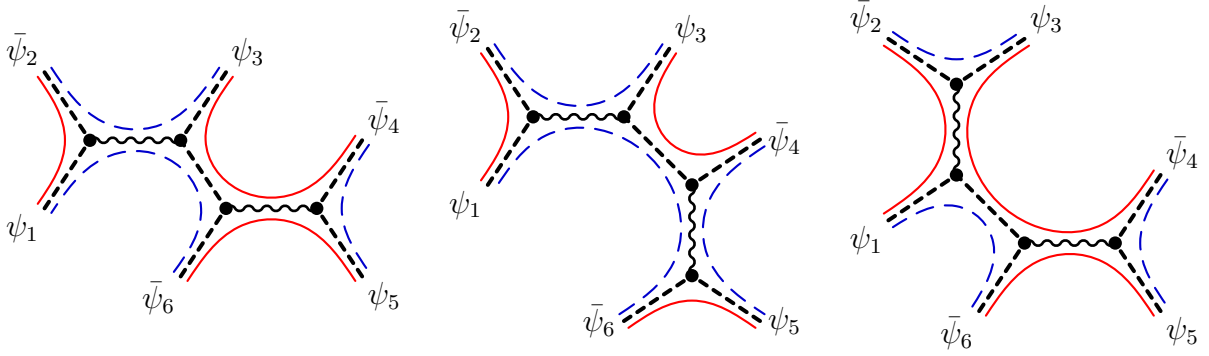
Figure 5: Diagram B, which contributes to the six-fermion amplitude. When color-stripped, the left diagram gives (D.8), and the other two diagrams equal the left one up to relabelings of the external legs.
