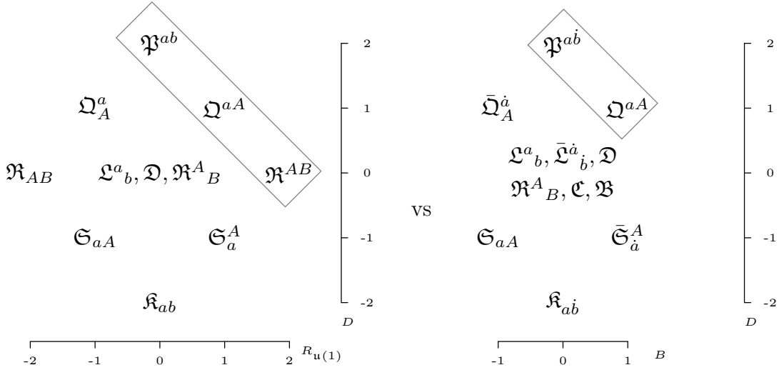
Figure 3: The symmetry generators of \mathfrak{osp}(6|4) (lhs) and \mathfrak{psu}(2, 2|4) (rhs). In \mathfrak{psu}(2, 2|4) the generators can be arranged according to their hyper- and dilatation charge. Similarly, we can arrange the generators of \mathfrak{osp}(6|4) if we replace the hypercharge by a u(1) R-symmetry charge. In \mathcal{N} = 4 SYM theory, the dual or level-one Yangian generators \mathfrak{P}^{(1)} and \mathfrak{Q}^{(1)} were identified with the generators \mathfrak{S}^{(0)} and \mathfrak{K}^{(0)} , respectively. The picture on the left suggests a similar dualization for \mathcal{N} = 6 SCS theory incorporating the R-symmetry.
