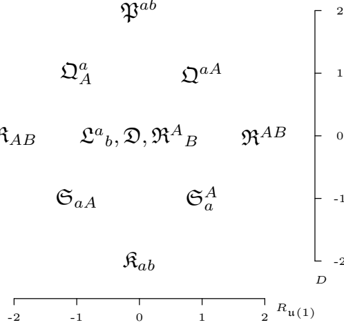
Figure 1: The generators of \mathfrak{osp}(6|4) can be arranged according to their dilatation charge and their \mathfrak{u}(1) charge under \mathfrak{R}^C_C .
