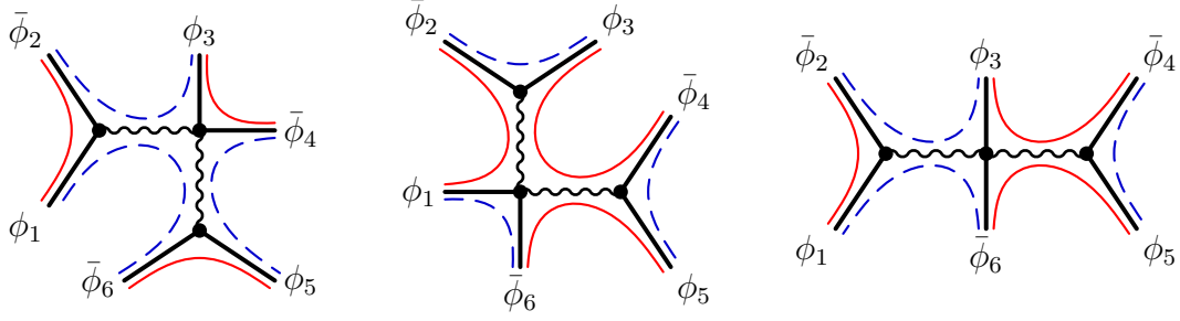
Figure 6: Diagram C that contributes to the six-scalar amplitude. Again, blue/dashed lines represent fundamental color contractions, red/solid lines represent antifundamental ones. When color-stripped, the left diagram gives (D.14), and the other two diagrams equal the left one up to relabelings of the external legs.
