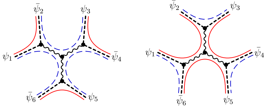
Figure 4: Diagram A, which contributes to the six-fermion amplitude. Blue/dashed lines represent fundamental color contractions, red/solid lines represent antifundamental ones. When color-stripped, the left diagram gives (D.6), and the right diagram equals the left one up to a relabeling of the external legs.
