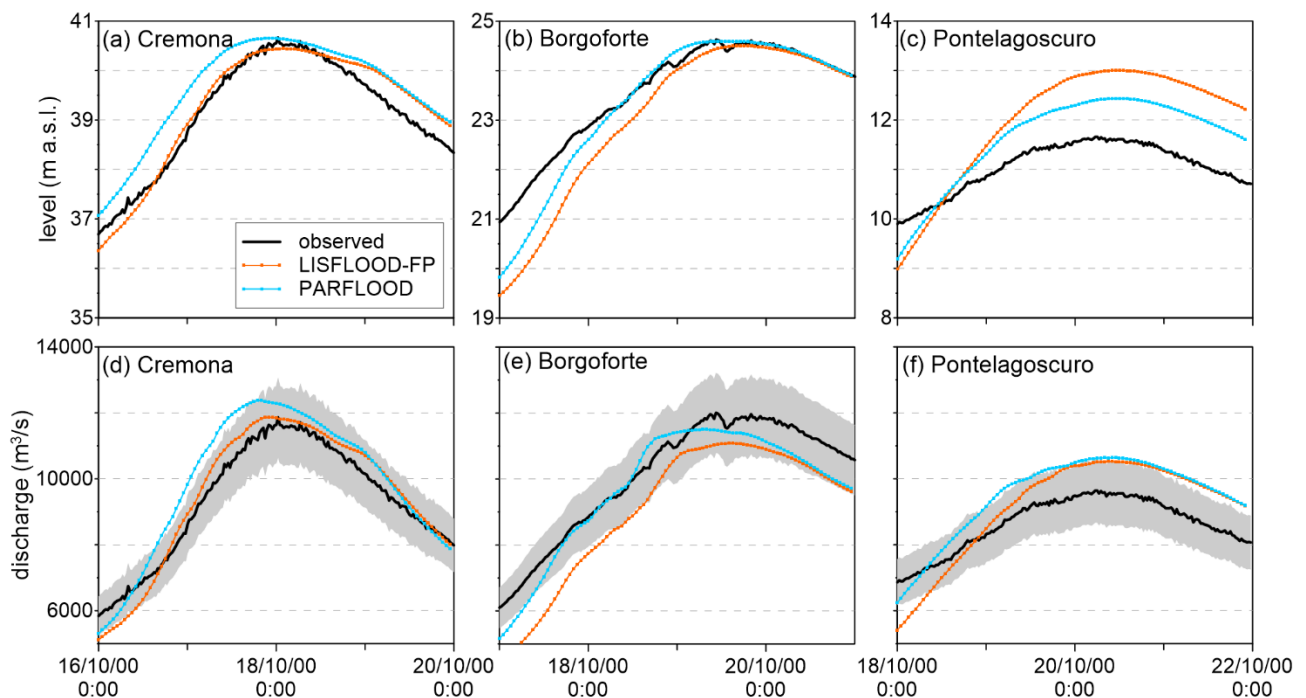
Figure 4 – Level (a-c) and discharge (d-f) time series in Cremona, Borgoforte, and Pontelagoscuro: comparison between measured values and simulations (30 m resolution) with PARFLOOD and LISFLOOD-FP. The grey band indicates an estimated 10% uncertainty on discharge observations. The time axis is reduced to improve readability.
