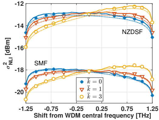
Fig. 5. NLI variance \sigma_{\text{NLI}}^2 versus frequency shift. Gaussian distributed symbols, 51 channels, 3 \times 100 km of SMFs or NZDSFs, without inline DGEs. Variable pre-emphasis factor \bar{k} , see Eq. (20). Solid: SSFM. Markers: Integral DGE-SRS-GN model. Dotted: extended-closed forms by using Eq. (20).
