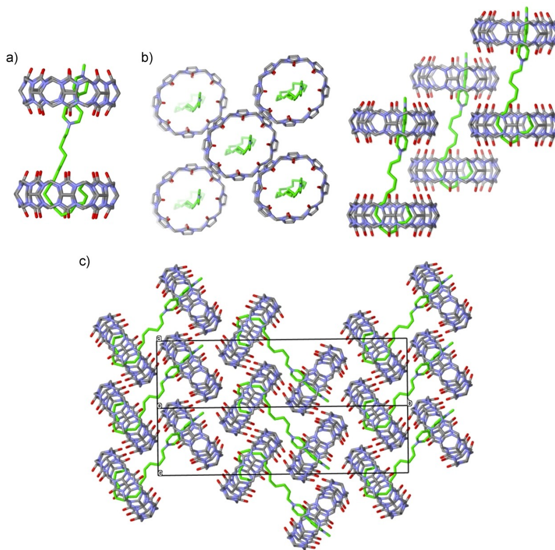
Figure 3. Stick representations of the crystal structure of \text{CB}[8]^+\text{MVC18} . a) side view of the 2:1 \text{CB}[8]^+\text{MVC18} complex presents in the asymmetric unit. b) orthogonal views of the square arrangement of the four 2:1 complexes surrounding the \text{MVC18} alkyl chain of the central 2:1 complex. Two pairs of the complexes are overlapped in the side view. c) Crystal packing, as viewed along the ac direction. The atomic species are represented in CPK colors with the exception of the \text{MVC18} carbon atoms, which are colored in green. Hydrogen atoms, water molecules and counter-anions are omitted for clarity.
