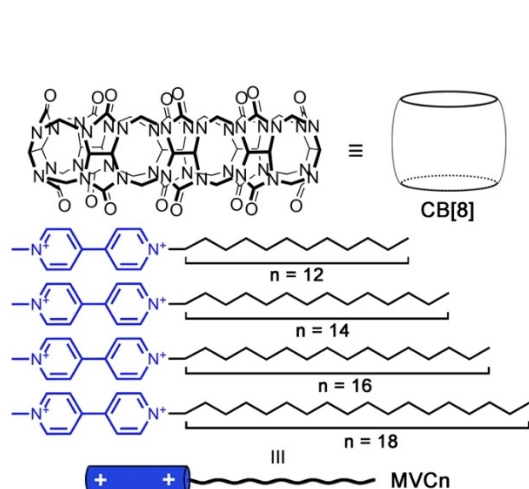
Scheme 1. Structure of cucurbit[8]uril ( CB[8] ) and methyl alkyl viologen dichloride salts ( MVCn ) involved in this study.
