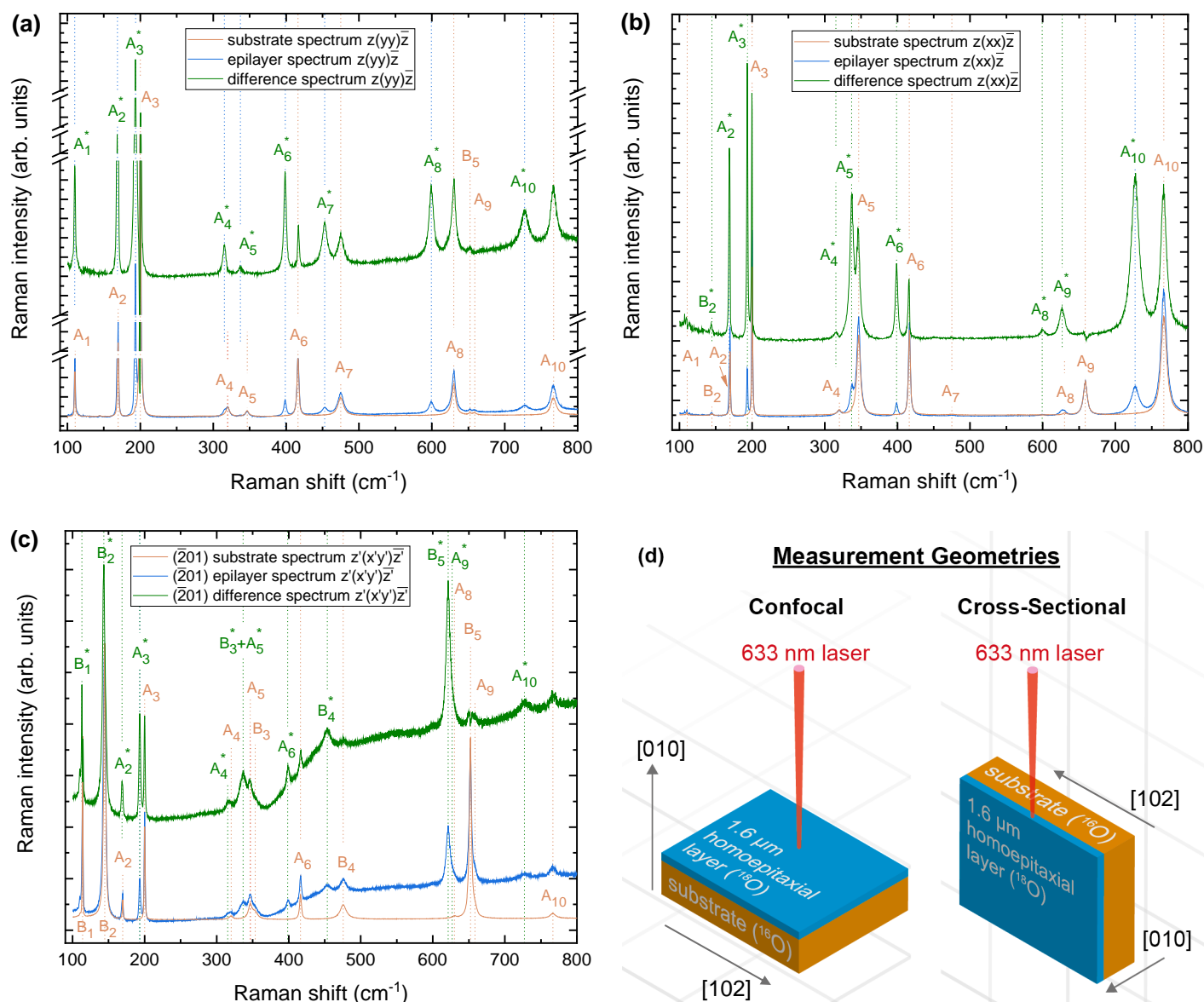
Fig. 2 Raman spectra of the homoepitaxially-grown \text{Ga}_2\text{O}_3 thin film ( ^{18}\text{O} ) on the (010) plane of a \beta\text{-Ga}_2\text{O}_3 substrate with natural ( ^{16}\text{O} ) isotope abundance. a,b ) Raman spectra in parallel polarization for excitation on the (010)-plane. Substrate spectra (dark yellow) were subtracted from the epilayer spectra (blue) to obtain difference spectra (green), in which ^{18}\text{O} Raman modes (denoted by *) dominate. For clarity, spectra are vertically offset and the difference spectra multiplied by a constant factor. The Cartesian coordinate system x,y,z is chosen such that z -axis aligns with the [010] direction, while y \parallel [100] . c ) Raman spectra of the (201)-plane in crossed polarization. The z' -axis is parallel to the surface normal, with x' \parallel [010] and y' \parallel [102] . d ) Schematic illustration of sample set-up, plane orientation, and measurement geometry. The (010) plane was accessible in confocal micro-Raman scattering (left). The [102] direction is oriented along an edge of the square-shaped wafer. Spectra of the (201)-plane were acquired by focusing the laser on the edge of the sample in cross-section geometry (right).
