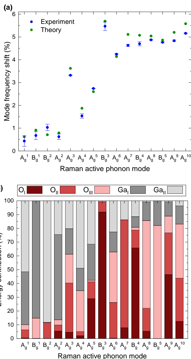
Fig. 3 (a) Relative mode frequency shifts of Raman modes for ^{18}\text{O} isotope substitution compared to natural isotope distribution based on experimental and theoretical data listed in Table 2. (b) Theoretical calculations of relative energy contributions to the total phonon energy corresponding to each O or Ga lattice site. Raman vibrations can be excited by one of the two Ga (grey) or one of the three O (red) lattice sites. The height of a column indicates the relative energy contribution of the corresponding lattice site.
